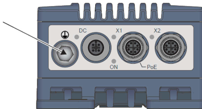
Figure 6. Earth connection
