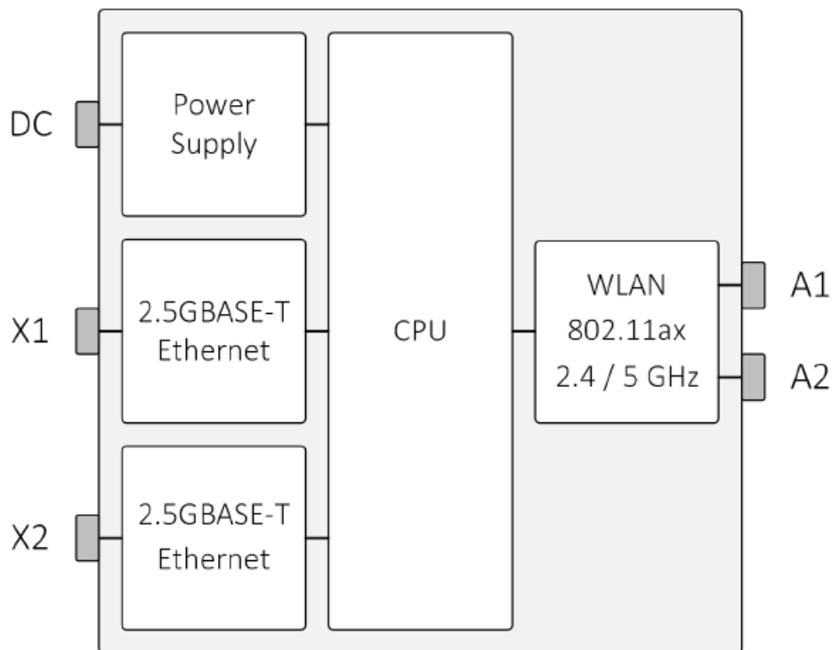
Figure 3. Ibex-1510 block diagram
