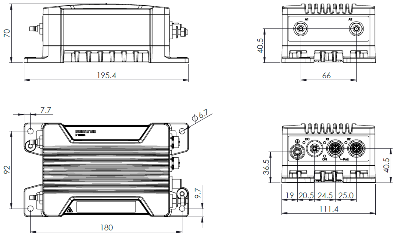
Figure 5. Dimensional drawing
