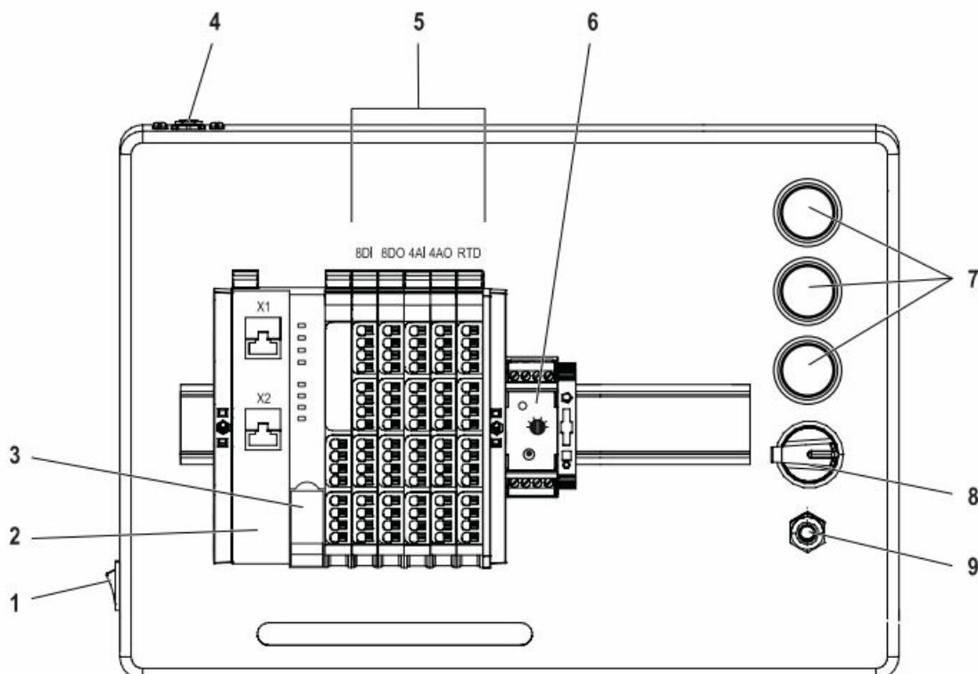
Figure 5: Overview of the starter kit hardware
