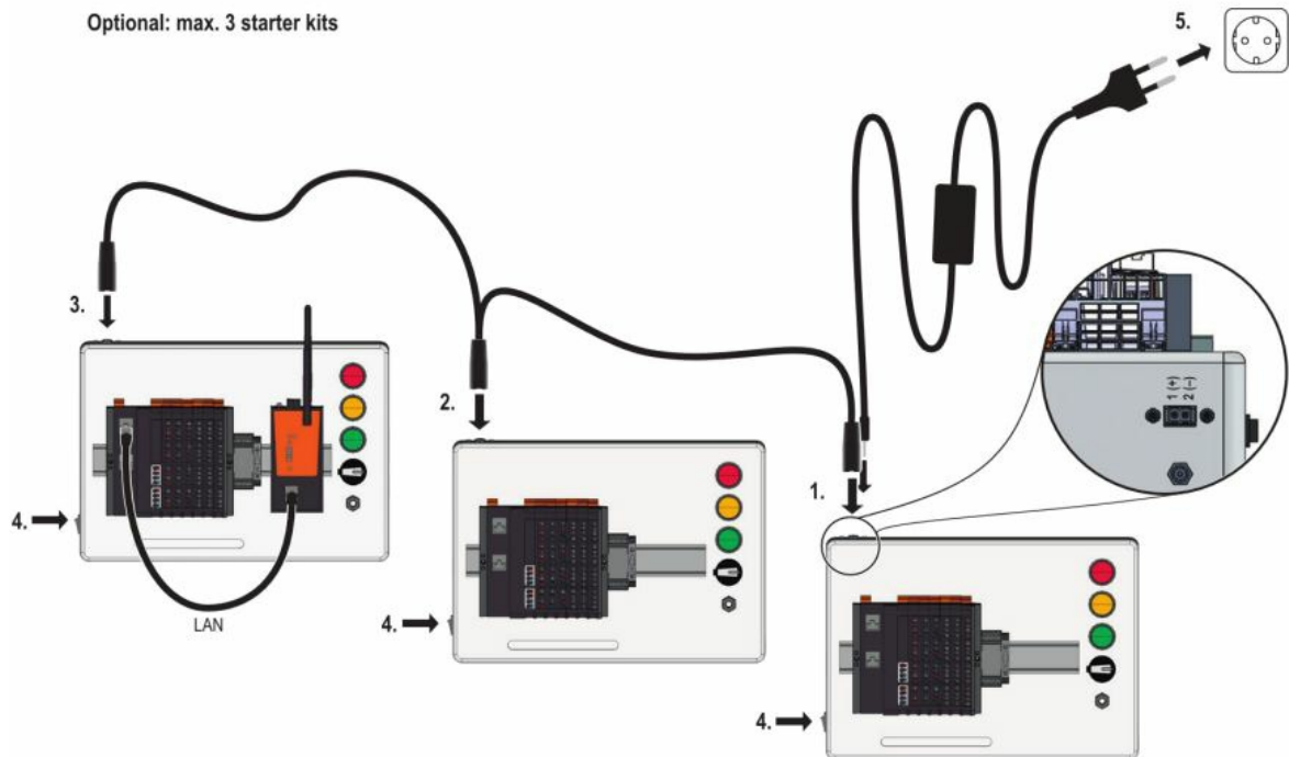
Figure 2: Daisy chaining of up to three starter kits
