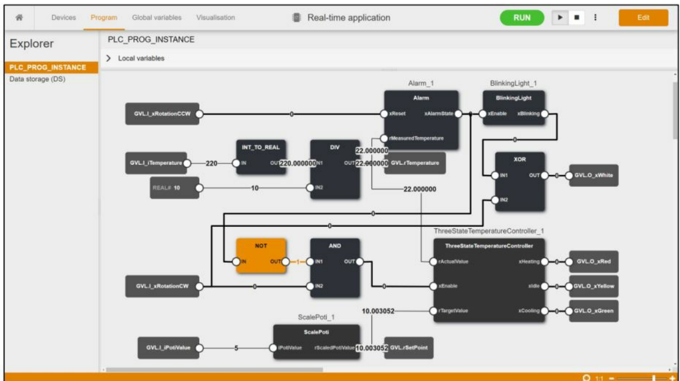
Figure 10: Live view of the PLC program in u-create web
