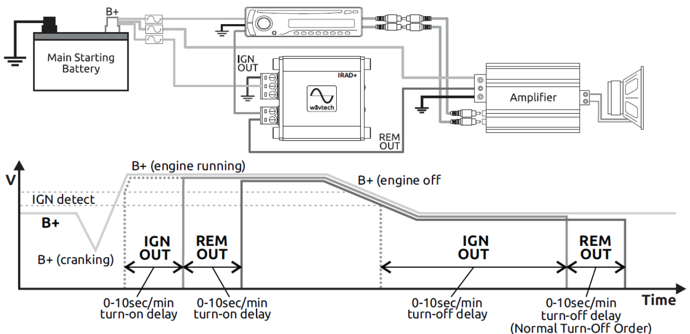
Example-1: Ignition Detect Mode w/Dual Outputs, Delays & Normal Turn-off Order
