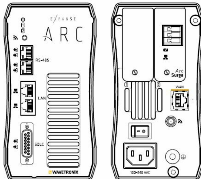
Figure 22. Arc faceplate (left) and backplate (right)
