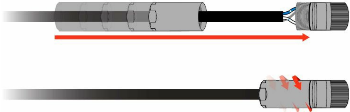
Figure 17. Tighten connector
