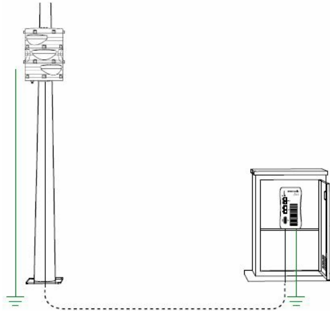
Figure 21. Typical XP21 installation
