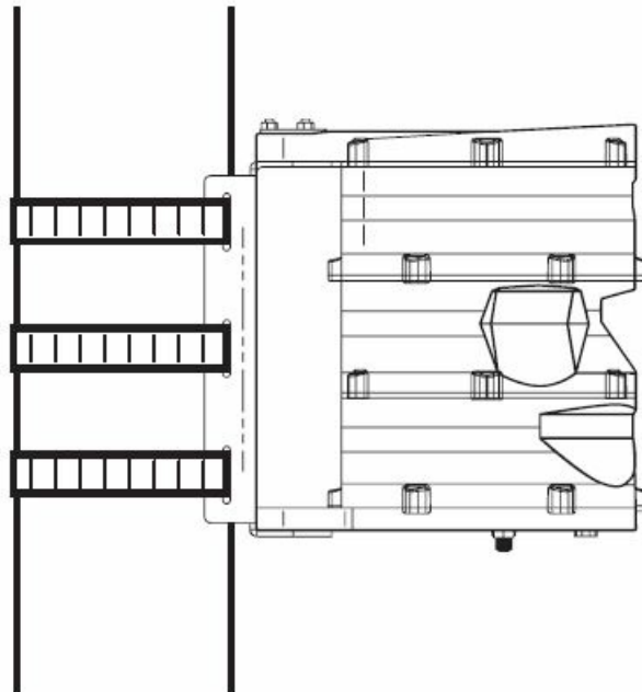
Figure 7. Tighten the nuts
