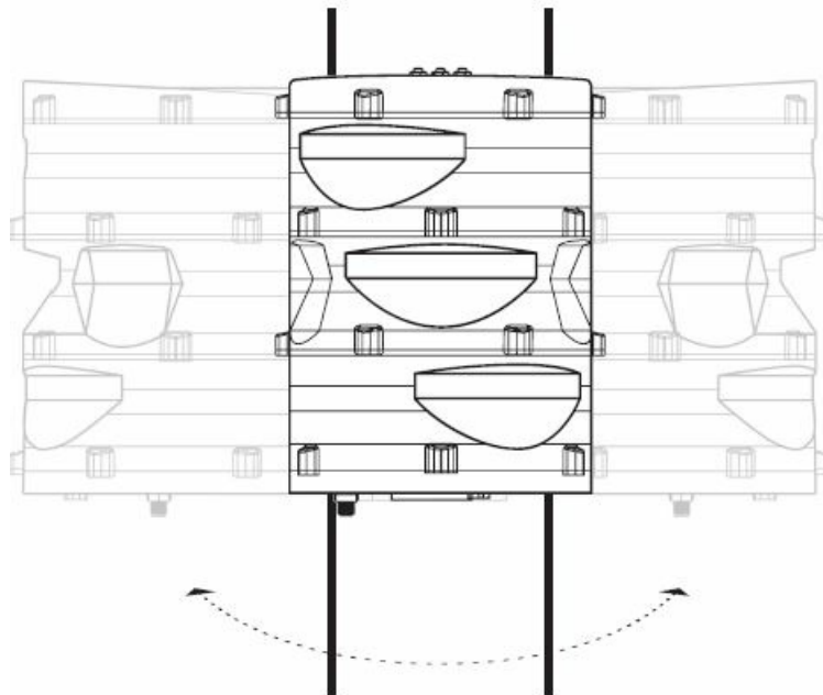
Figure 8. Aligning the sensor
