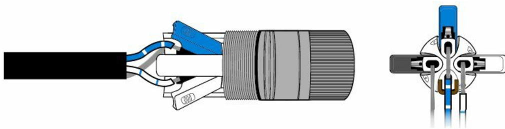
Figure 15. Terminate conductors in pin housing
