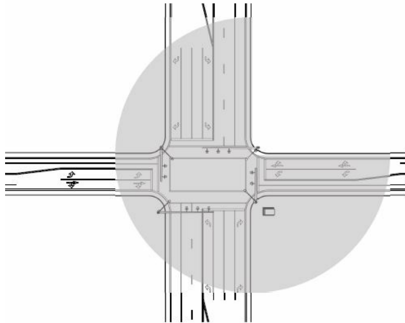
Figure 2. XP21 footprint's 120-ft. (36.5-m) range
