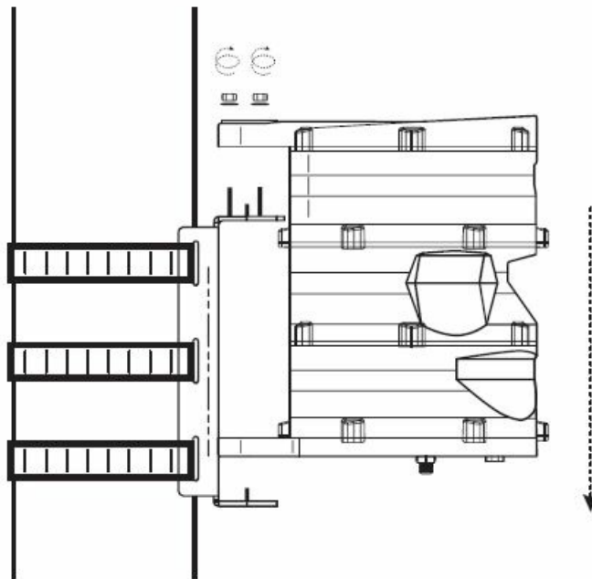
Figure 6. Mounting the sensor
