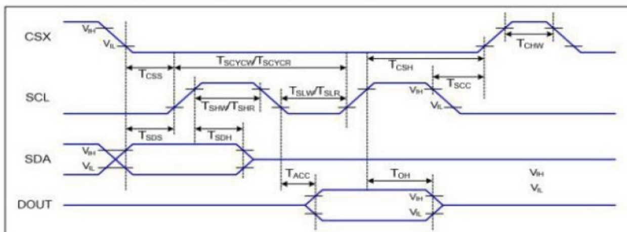
Figure 1 3-line serial Interface Timing Characteristics
