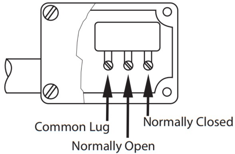
Single Pole Double Throw Switch
