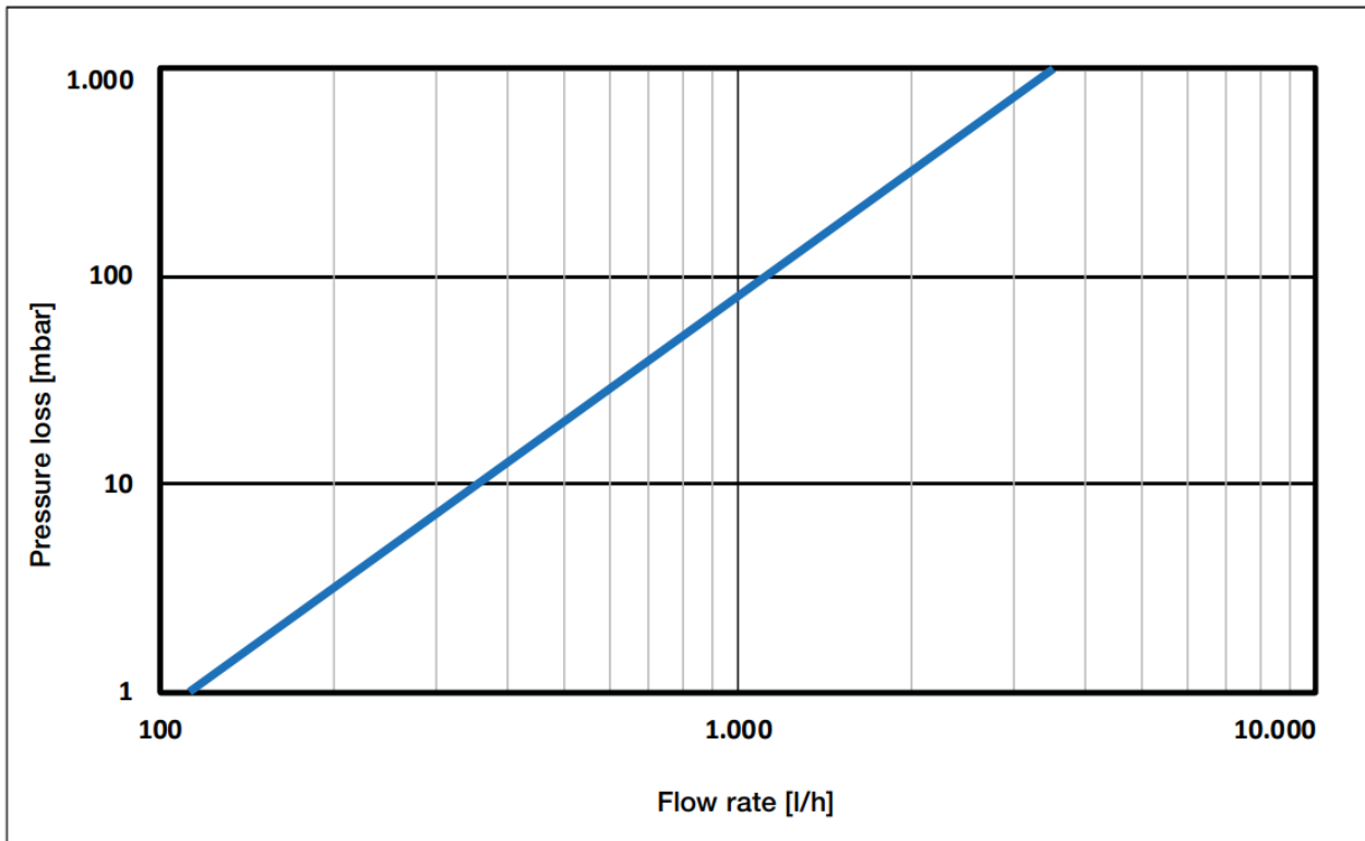
Fig. 7-1 Pressure loss diagram
