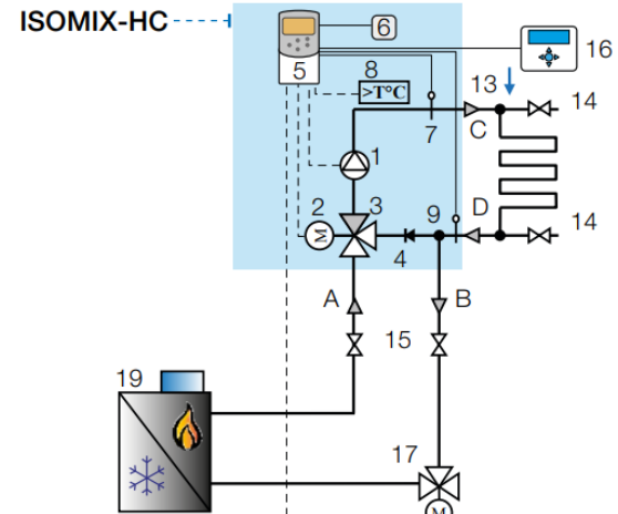
System diagram of radiant panel heating/cooling Reversible heat pump
