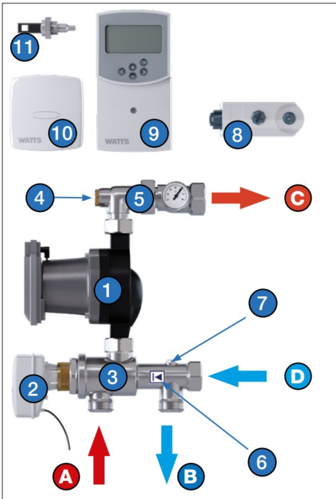
Fig. 3-1 Structure
