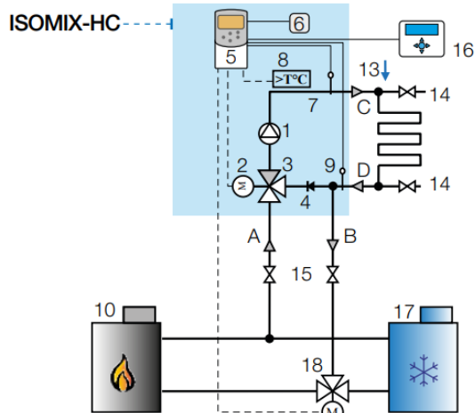
System diagram of radiant panel heating/cooling Separated boiler and chiller.
