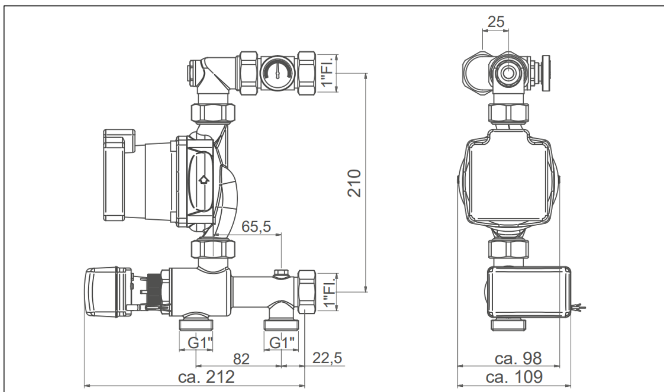
Fig. 6-1 Overall dimensions
