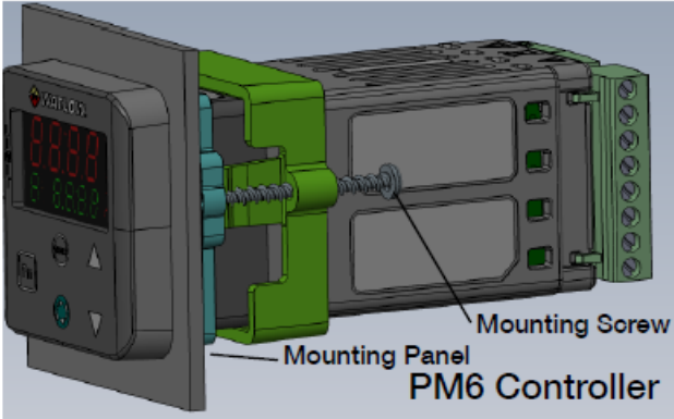
Figure 1: PM6 Installation
