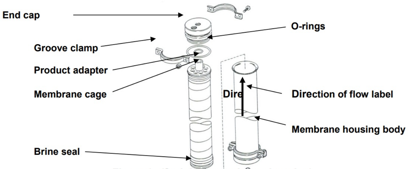
Figure 3. (Stainless membrane housing)
