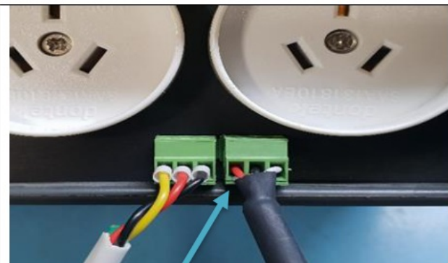
From right-hand port of Exp Unit 2...
