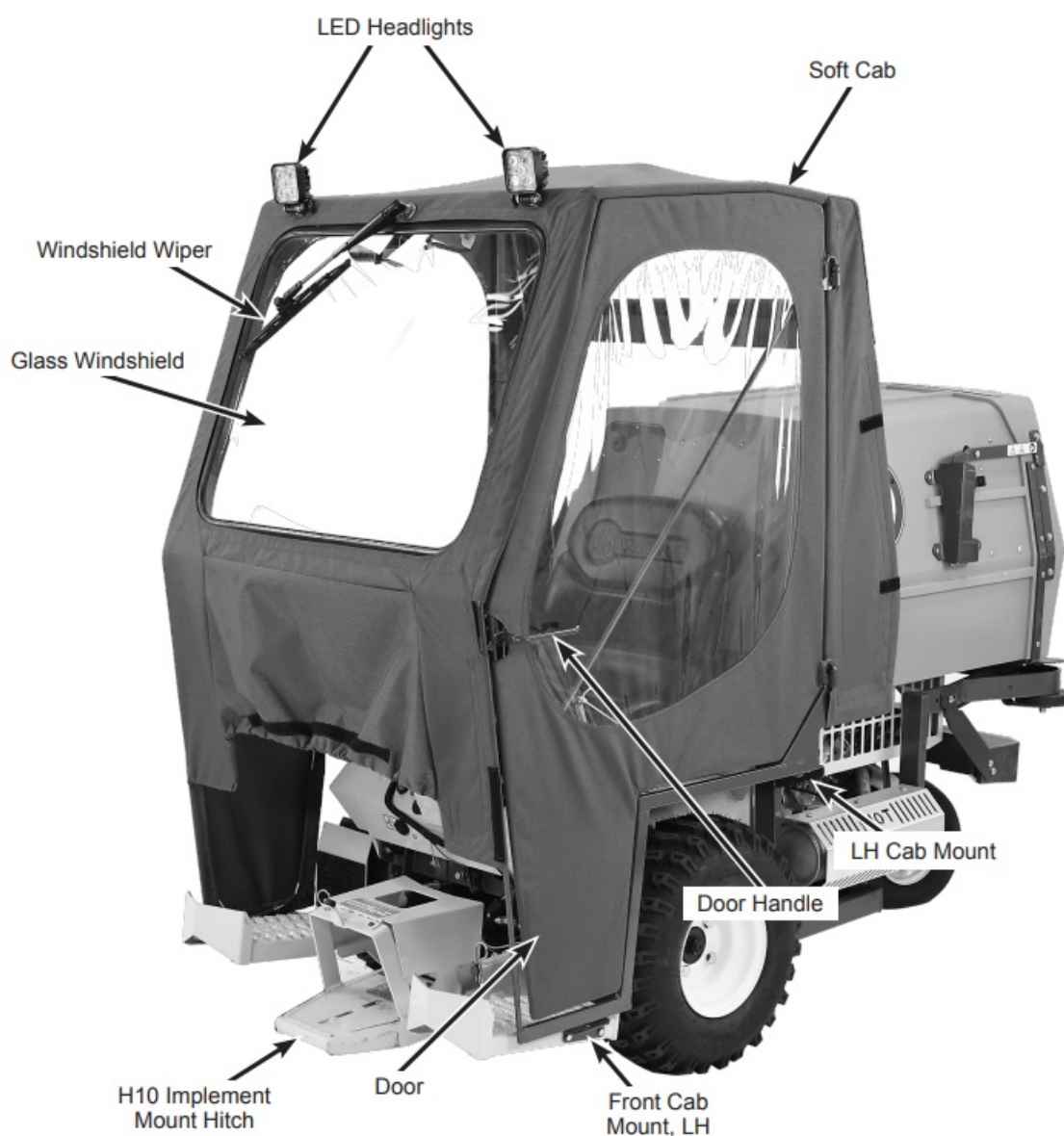
A13 Operator Soft Cab, LH View
