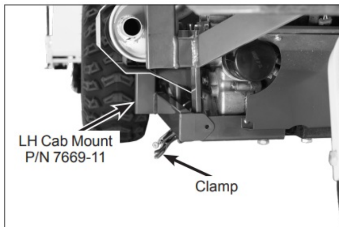
LH Cab Mount Installation
