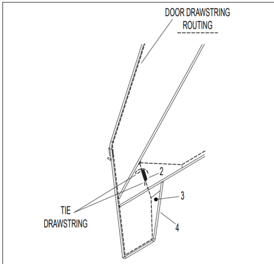
Soft Cab Door Drawstring Routing
