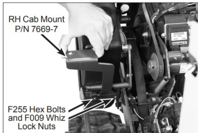
RH Cab Mount Installation
