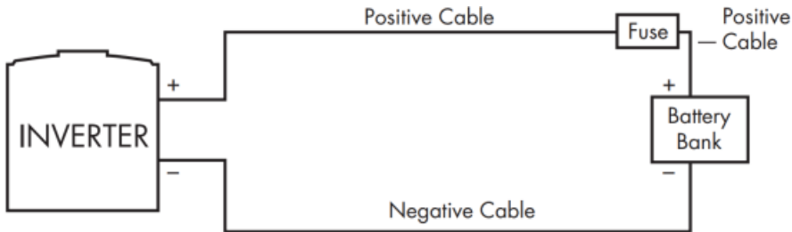
Total Cable Length for Home and Vessel Use
