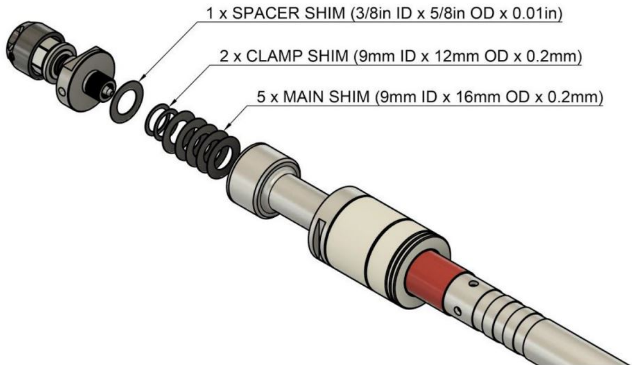
DRAWING 3: Stock shim stack configuration
