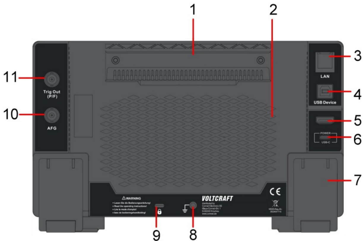
Figure 3-2: Rear Panel
