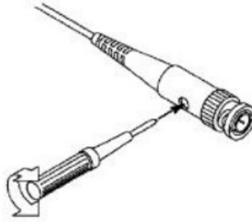
Figure 3-6: Adjust Probe
