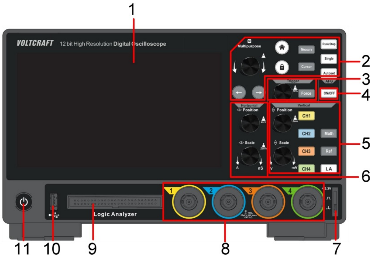
Figure 3-1: Front panel
