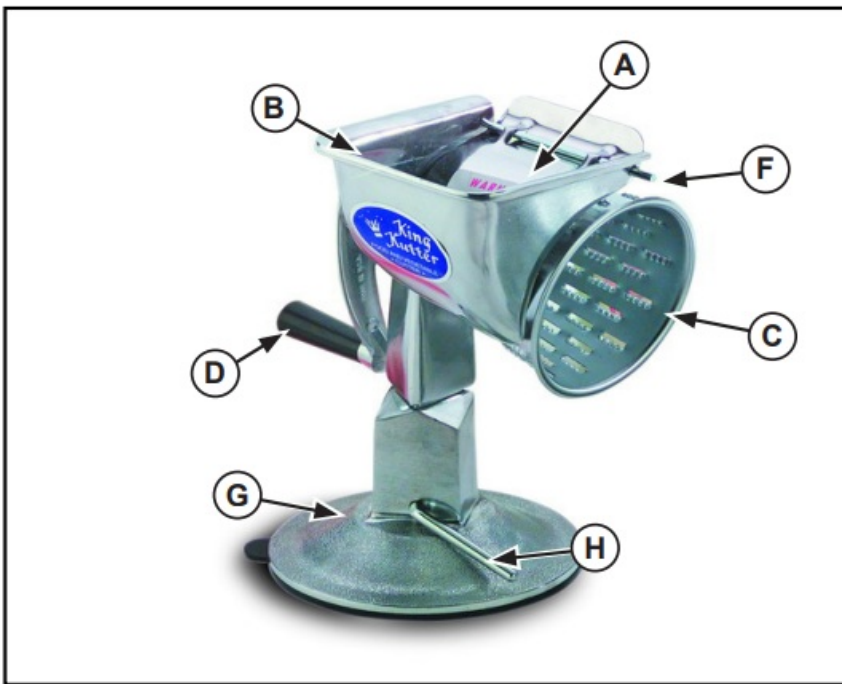
Figure 2. Features and Controls Suction Base.
