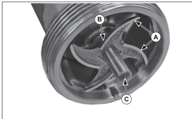
Figure 5. Knife Blade and Blade Shaft
