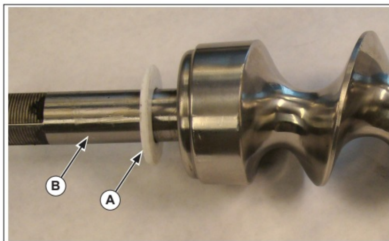
Figure 2. Shaft Washer and Worm Gear Shaft
