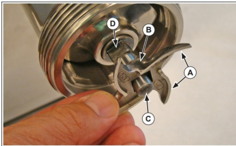
Figure 4. Knife Blade and Blade Shaft
