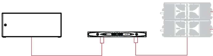
Figure 4.4: 1 x Arcline 218 and 2 x Arcline 8: 8 \Omega per channel / 1 amplifier
