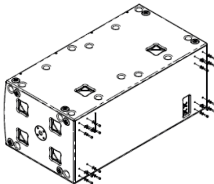
Figure 5.3: Bolt tightening
