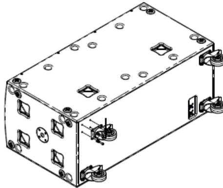
Figure 5.2: Wheel removal
