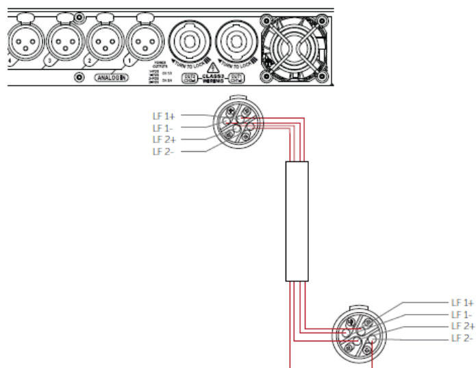
Figure 4.4: Bias Q5
