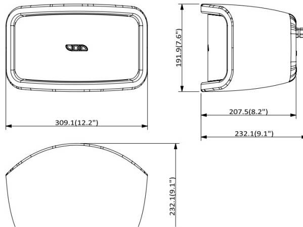
Figure 3.3: Dimensions
