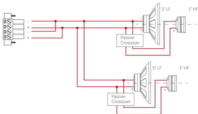
Figure 4.7: Wiring diagram
