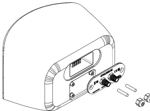
Figure 4.3: Glanded connector removal
