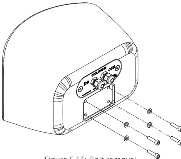
Figure 5.13: Bolt removal
