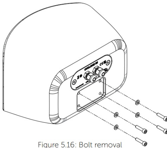
Figure 5.16: Bolt removal
