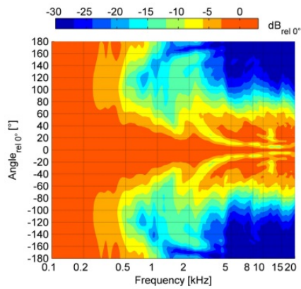
Figure 3.1: Horizontal directivity isobars
