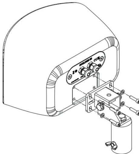
Figure 5.17: Pole mount kit attachment
