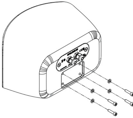
Figure 5.2: Bolt removal
