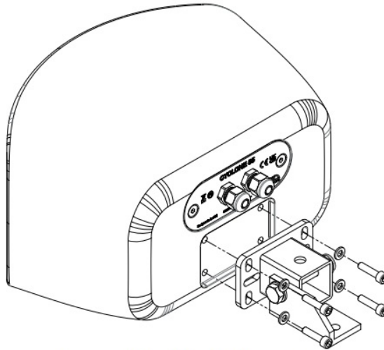
Figure 5.12: T51 stud bracket
