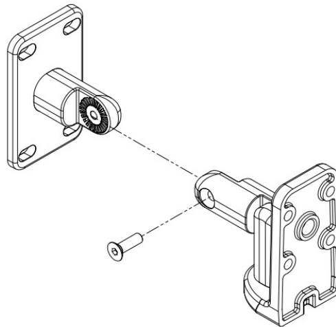
Figure 5.3: Mounting plate
