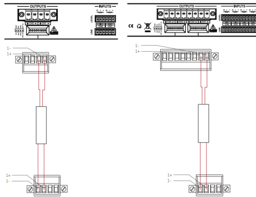
Figure 4.8: Bias D1 output connection
