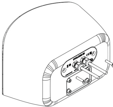
Figure 4.5: Phoenix attachment
