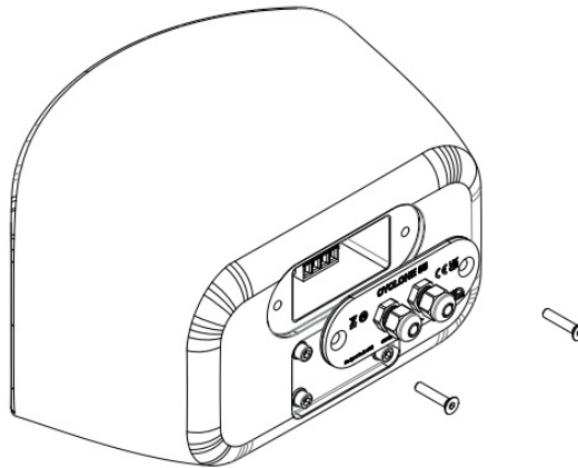
Figure 4.2: Connector plate removal
