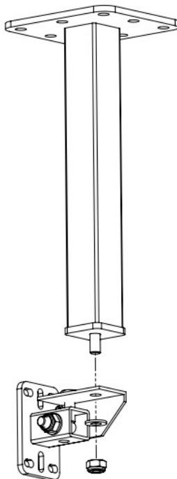
Figure 5.8: Mounting plate removal
