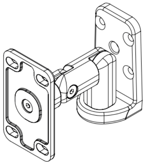
Figure 5.1: T51 bracket
