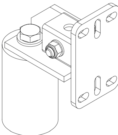
Figure 5.15: T51 pole bracket kit
