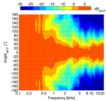
Figure 3.2: Vertical directivity isobars
