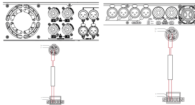
Figure 4.10: Bias Q3
