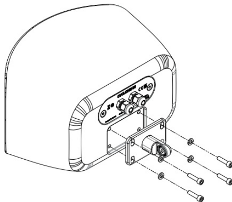
Figure 5.4: Bolt attachment
