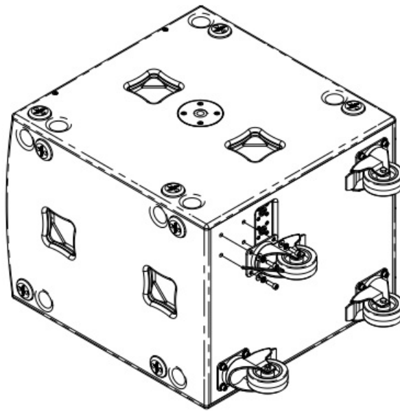
Figure 5.2: Wheel removal
