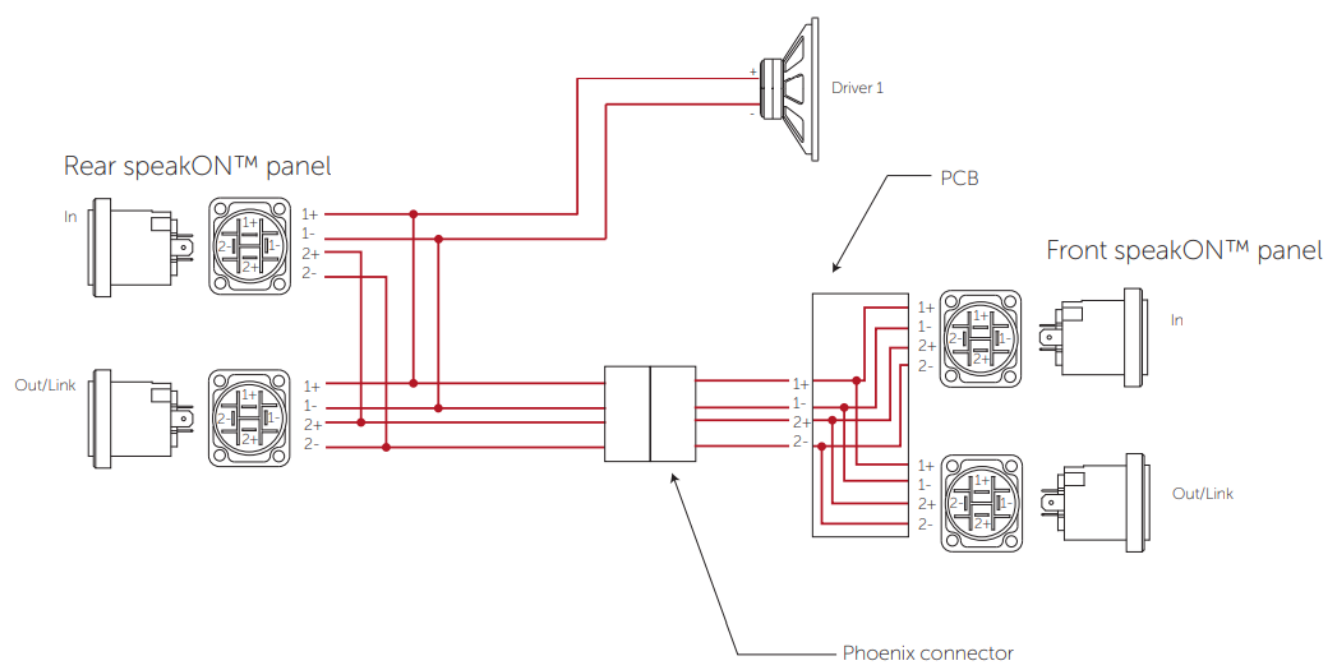
Figure 4.2: Wiring diagram
