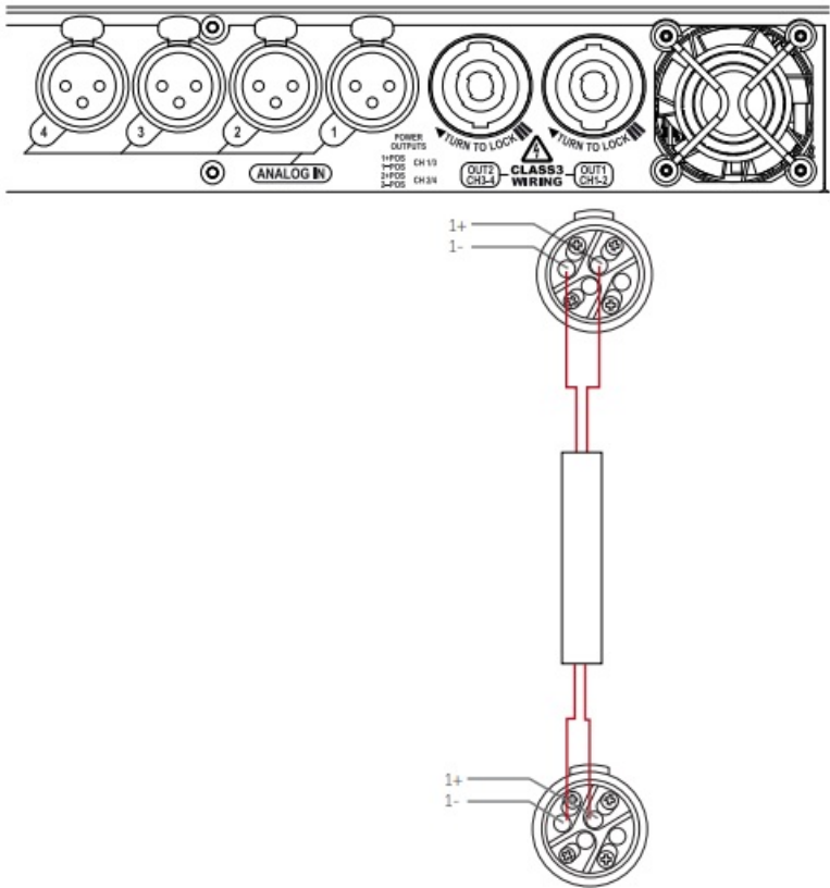
Figure 4.3: Bias Q5
