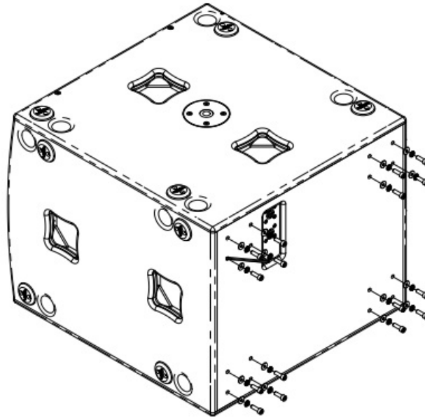
Figure 5.3: Bolt tightening
