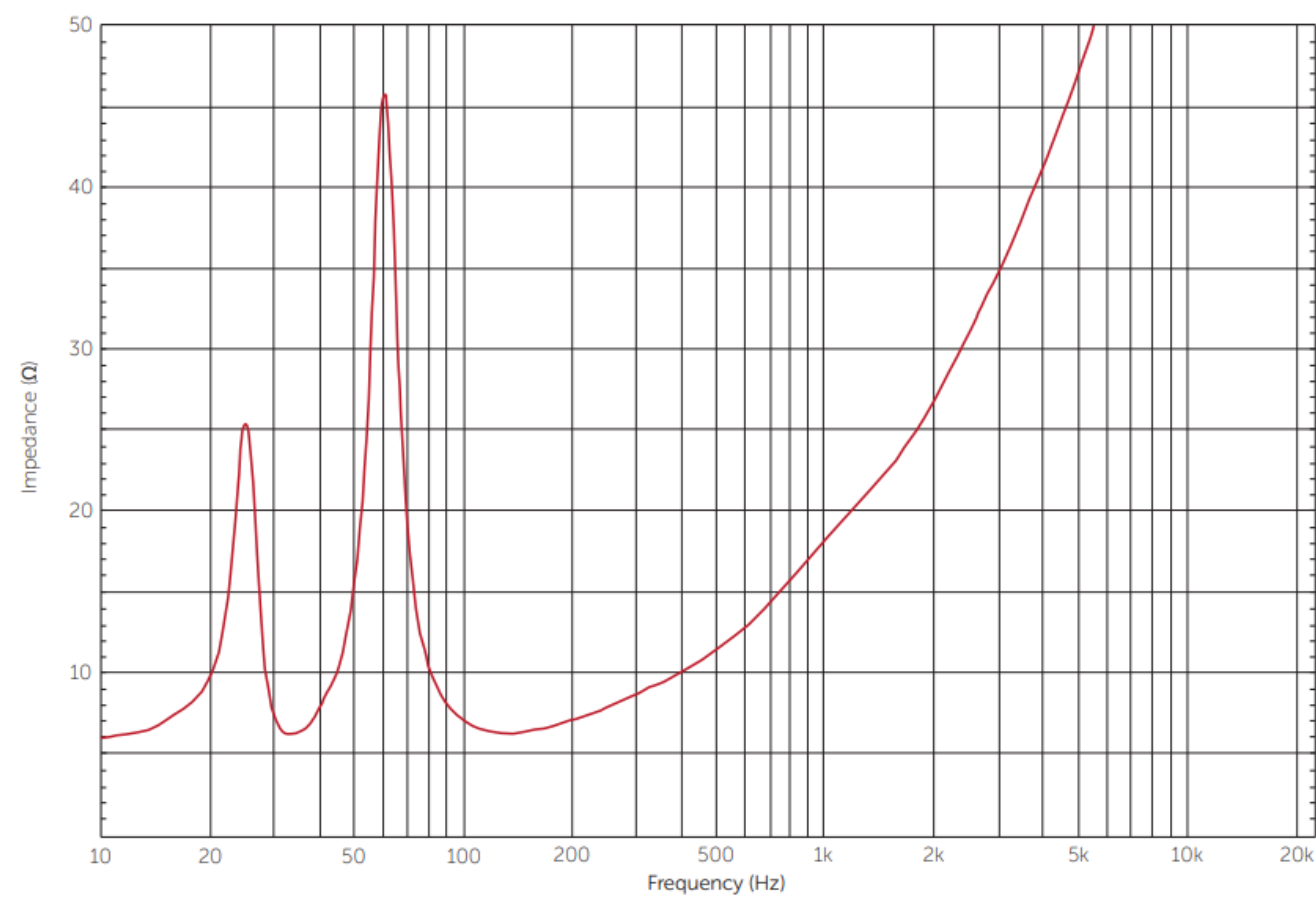
Figure 4.1: Impedance graph
