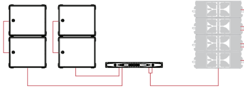
Figure 4.5: 2 x Arcline 118 and 4 x Arcline 8: 4 \Omega per channel / 1 amplifier
