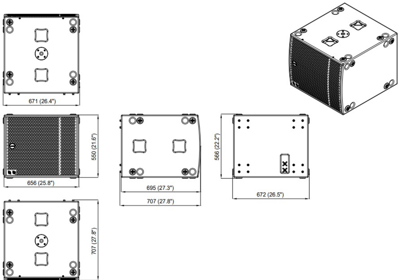
Figure 3.1: Dimensions
