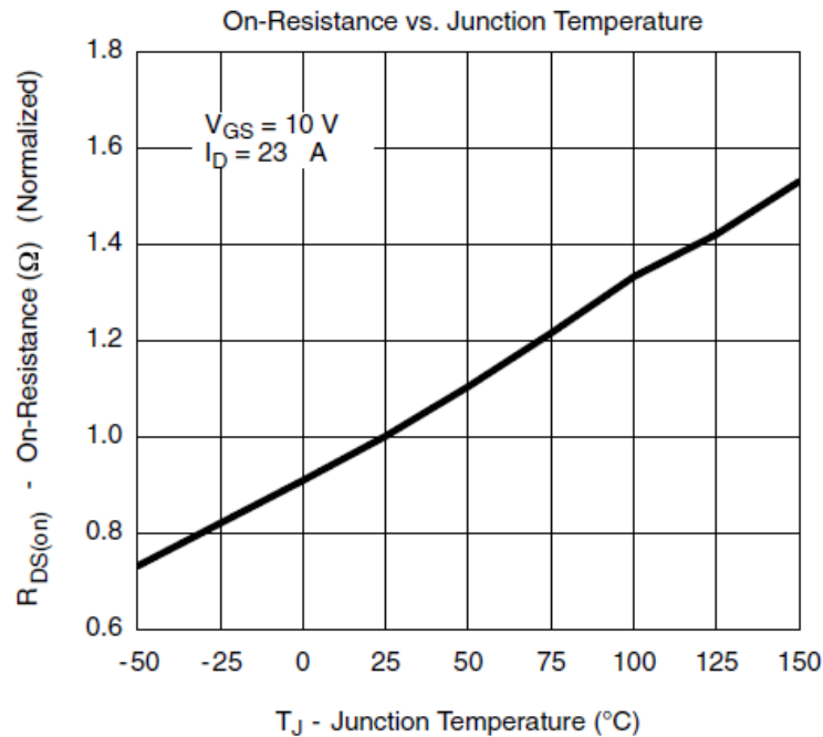
Fig. 7 MOSFET R_{DS(on)} vs. Temperature
