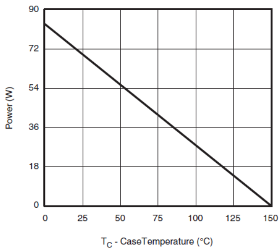
Power, Junction-to-Case
