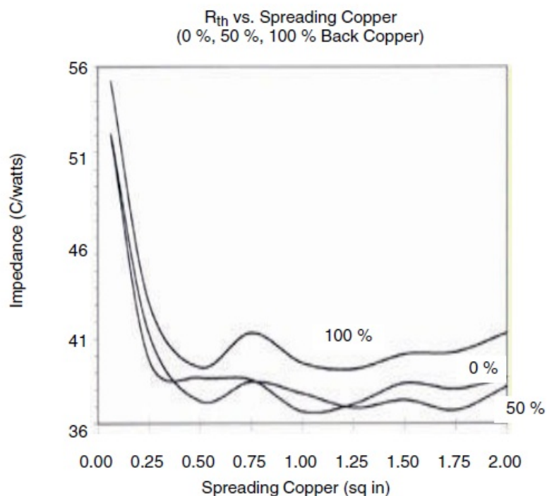
Fig. 6 Spreading Copper Junction-to-Ambient Performance
