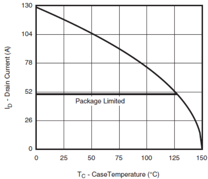
Current Derating a
