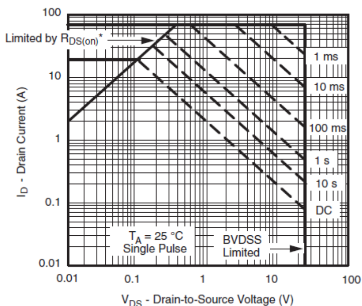
Safe Operating Area, Junction-to-Ambient
