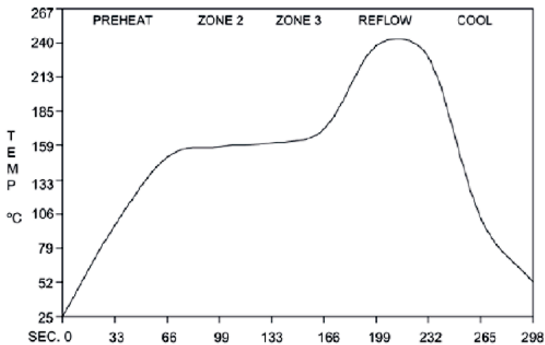
Fig. 3 Solder Reflow Temperature Profile
