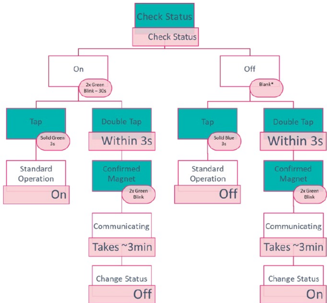
Flow Diagram for Cycling System Status with Magnetic Key
