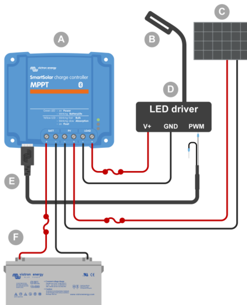
Wiring example - Controlling a streetlight LED driver.
