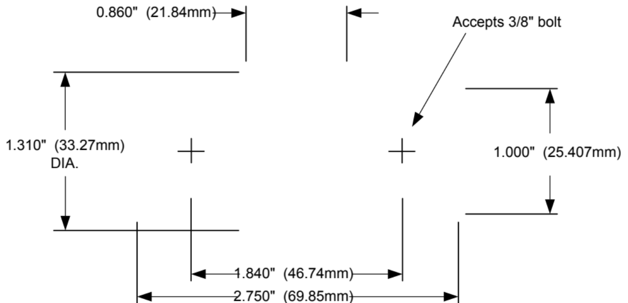
Class-T fuse dimensions in inches (mm)
