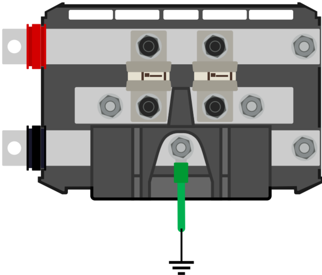
Ground connection Lynx Class-T Power In
