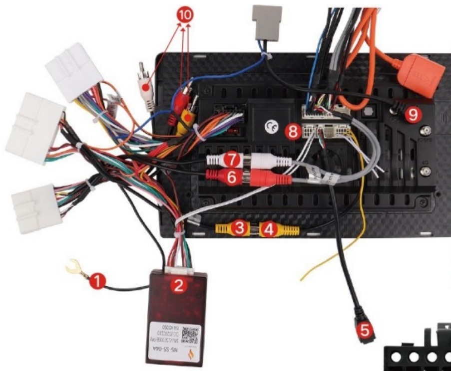
Wiring harness connection diagram
