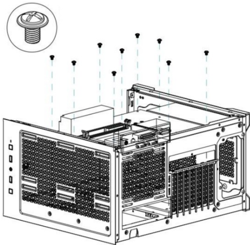
Installing the motherboard
