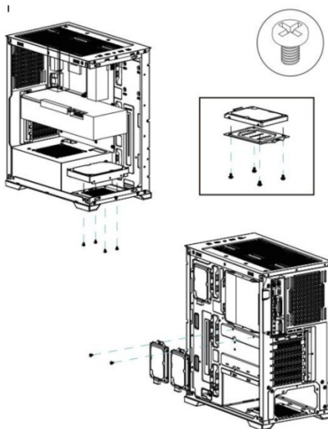
Installing SSD and HDD hard drives
