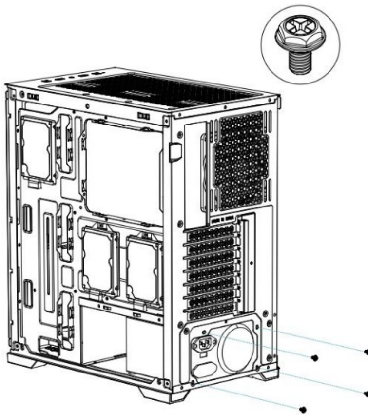
Installing power supply
