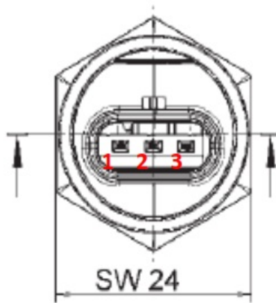
Sensor plug Female, product side view
