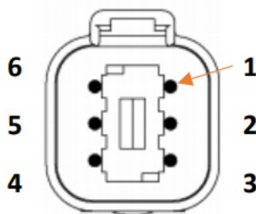
Deutsch DT04-6P plug, front view
