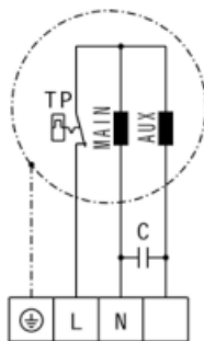
Wiring diagram EMF35512** EMF35514**
