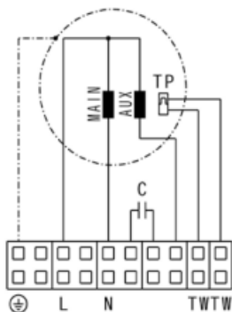
Wiring diagram EMF45014** EMF50014** EMF56014** EMF63014**
