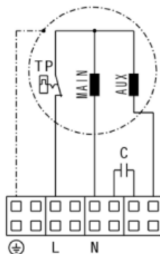
Wiring diagram EMF40014
