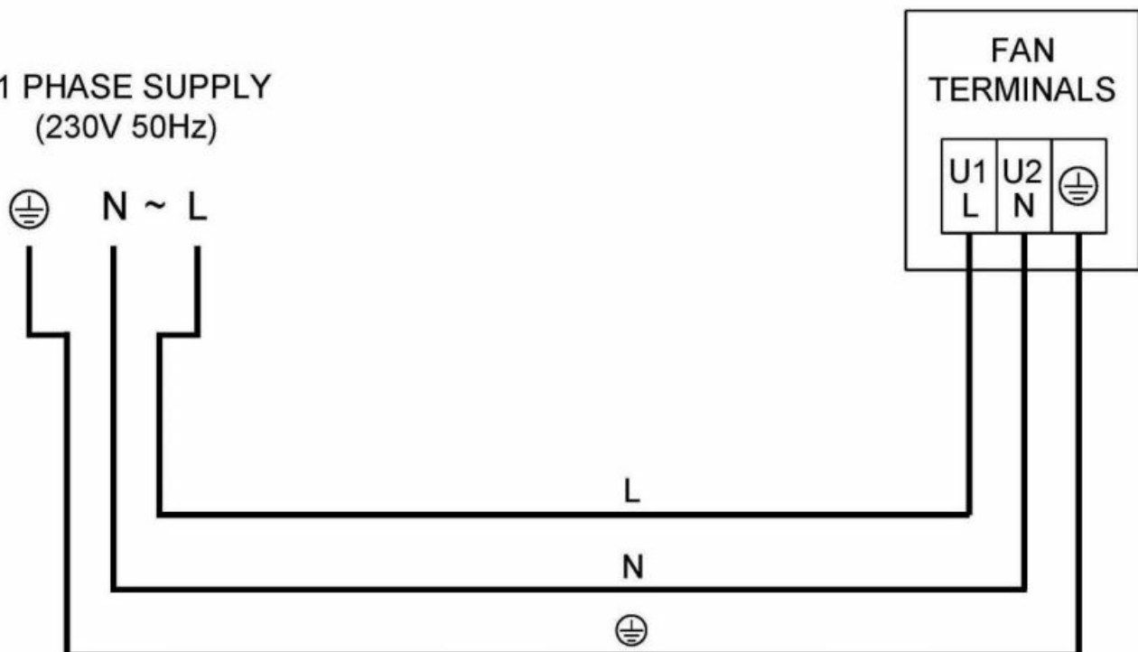
Fig. 2 ACQ20012D, ACQ25012D, ACQ31512LD. *Note; this diagram is not applicable to ACQ31514HD! Supply connections
