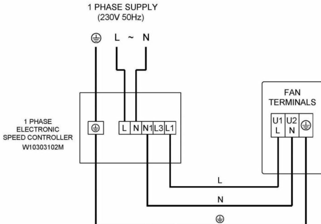
Fig. 4 ACQ20012D, ACQ25012D, ACQ31512LD. Connected to an electronic controller
