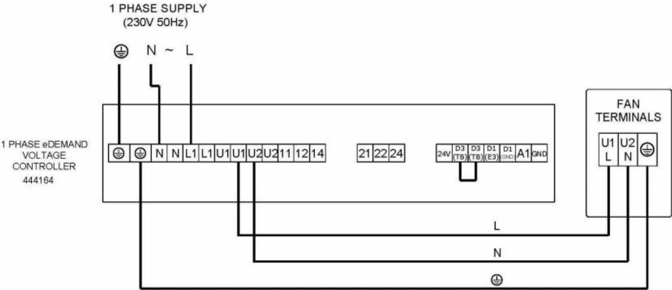
Fig. 14 ACQ40014D, ACQ50014D. Connected to an eDemand voltage controller
