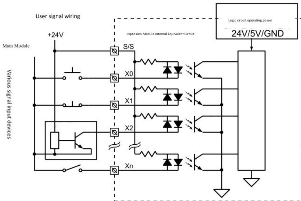
Figure 3-1 I/O expansion module internal equivalent input circuit Figure 3-1 I/O expansion module internal equivalent input circuit
