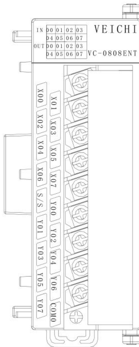
Figure 1-4 VC-0808ENT appearance and terminal diagram
