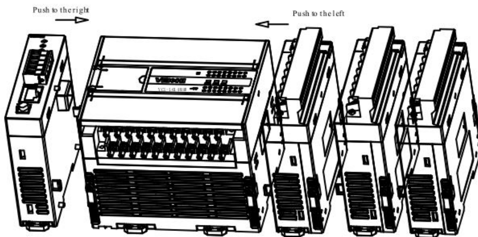
Figure 5-1 Extension module cascading method
