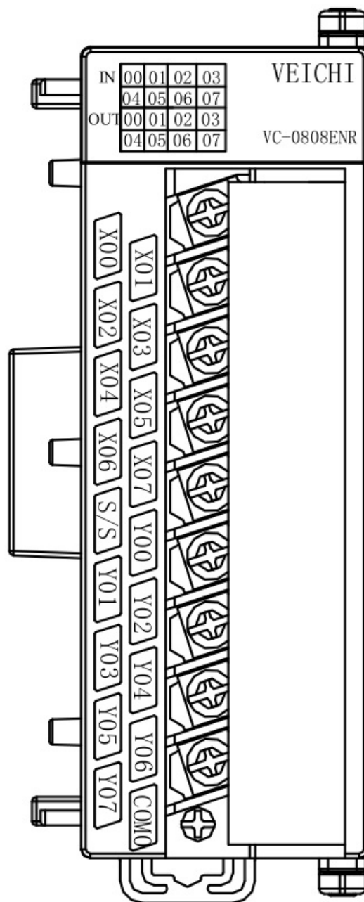
Figure 1-3 VC-0808ENR external appearance and terminal diagram
