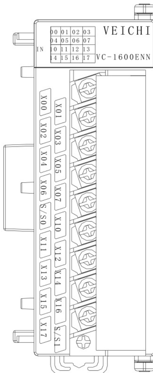
Figure 1-7 VC-1600ENN Outline and Terminal Diagram
