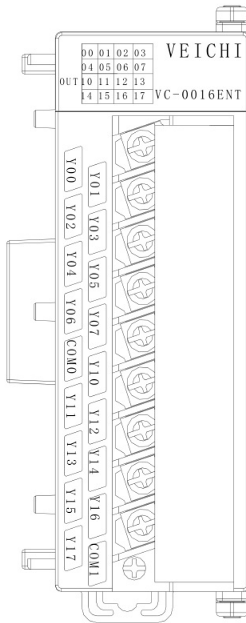
Figure 1-5 VC-0016ENT appearance and terminal diagram
