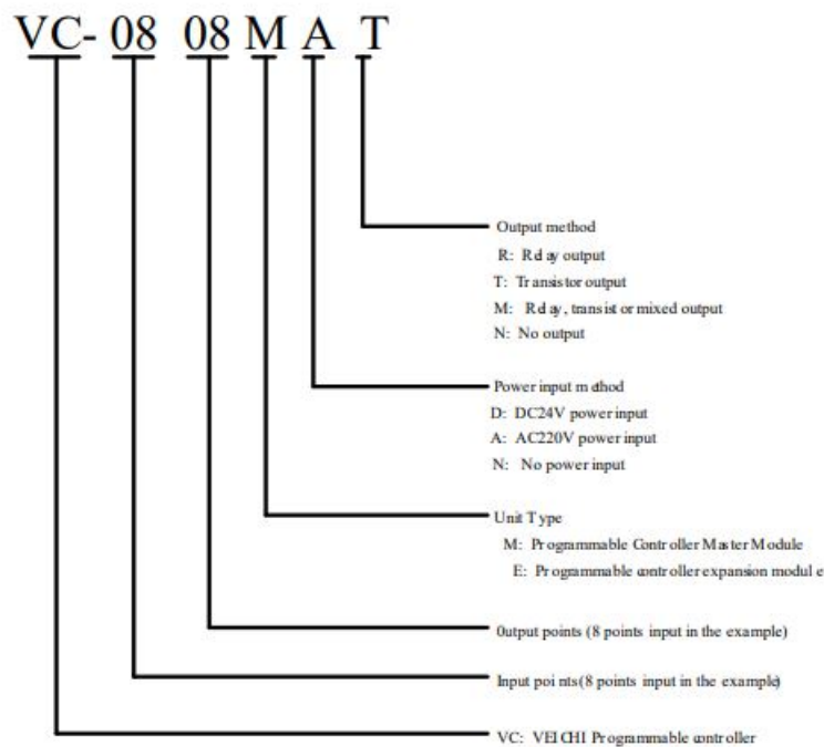
Figure 1-2 PLC model description
