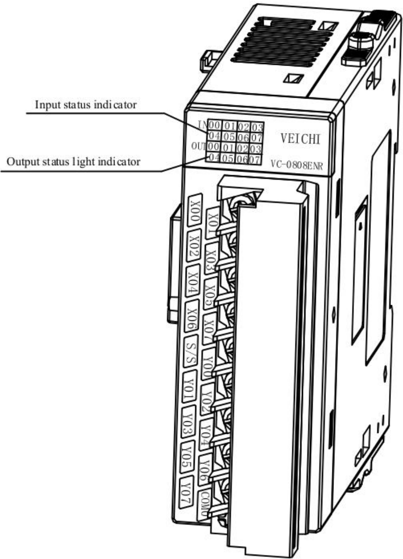
Figure 3-2 I/O expansion module status indicators
