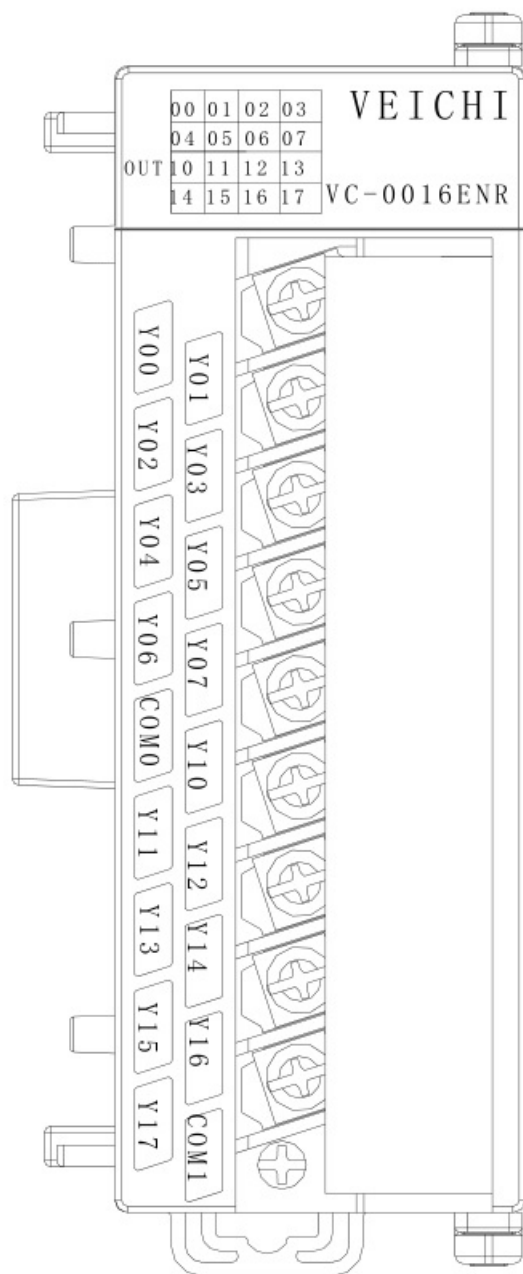
Fig. 1-6 VC-0016ENR external and terminal diagram
