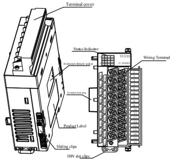
Figure 1-1 I/O expansion module form factor and components
