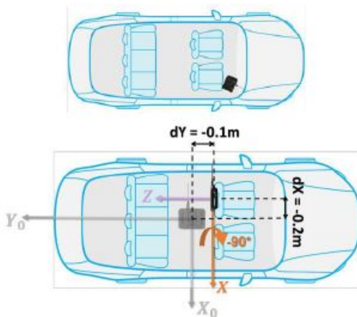
Figure 13: 90 Degree Back-seat Installation – Top view
