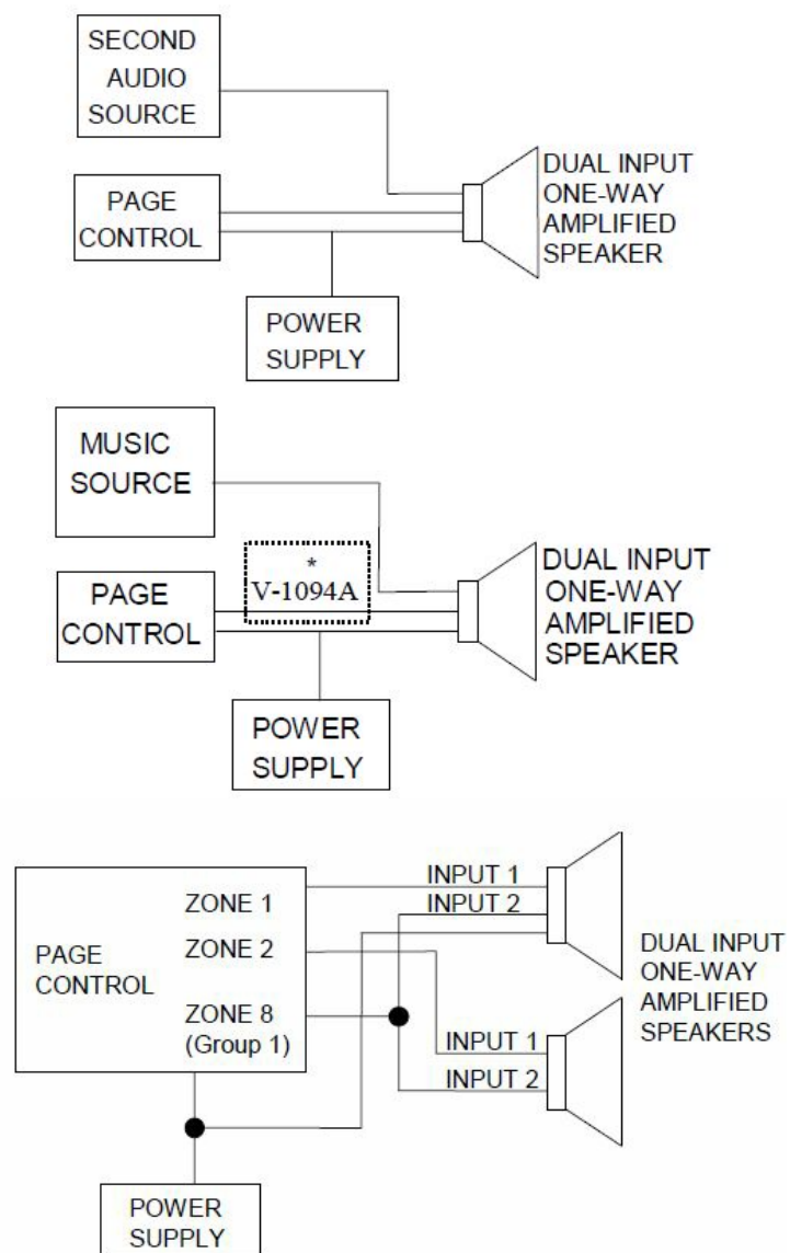
FIGURE 3 - GROUP CALL BLOCK DIAGRAM
