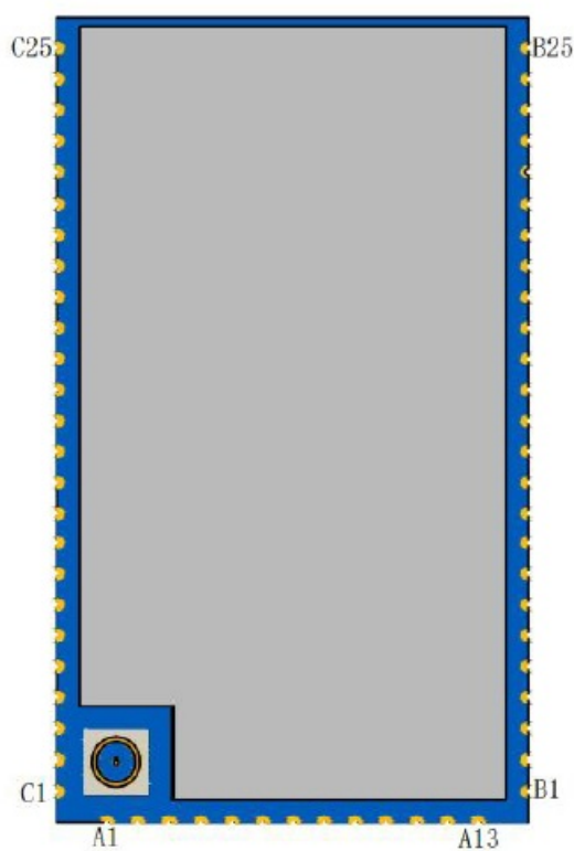
Pic 3 Pin definition
