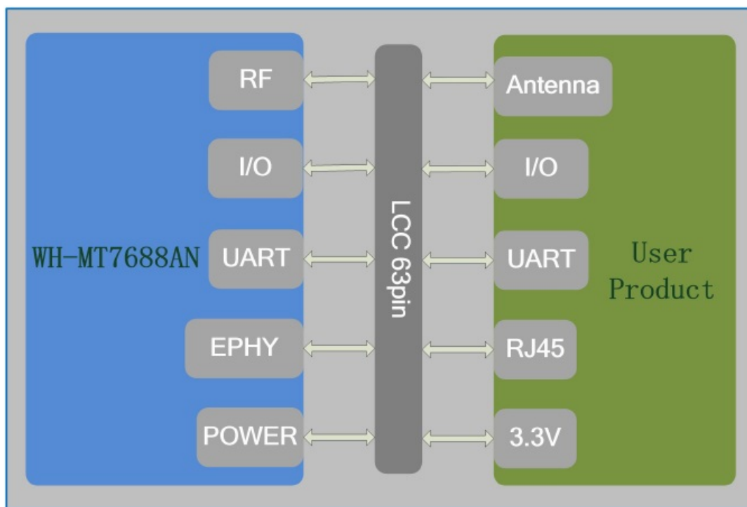
Pic 2 Block diagram of the module application
