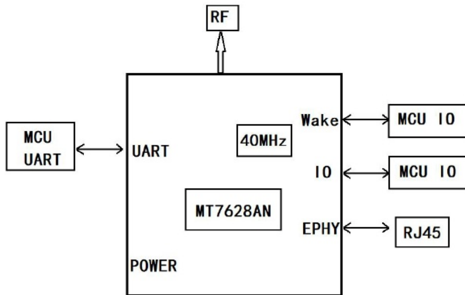
Pic 4 Module peripheral circuit reference
