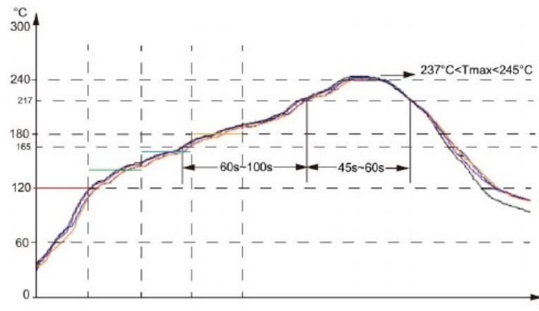
Pic5 A reflow temperature profile is recommended
