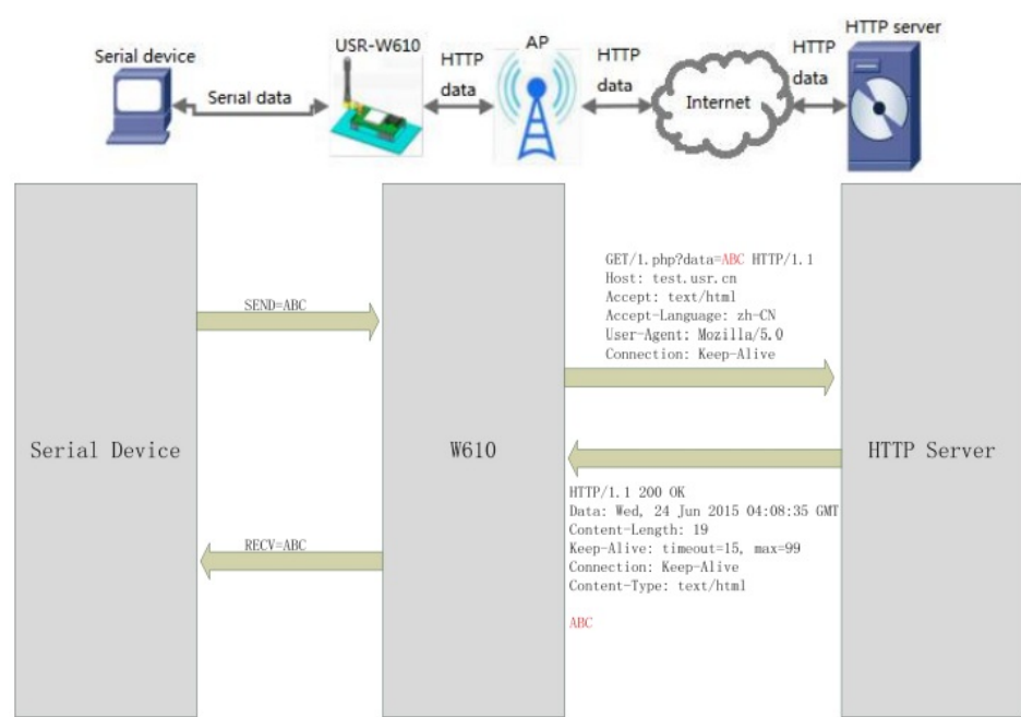
Figure 14 HTTP Client mode
