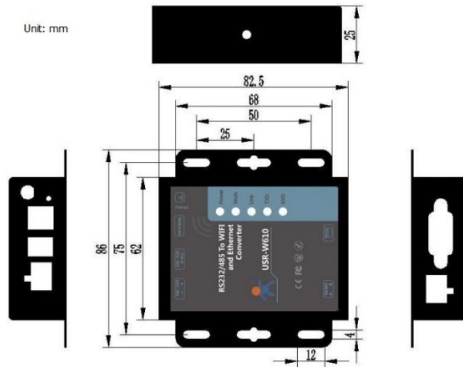
Figure 4 Dimension
