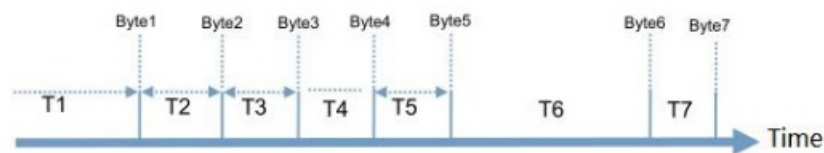
Figure 17 Serial Free-Frame mode
