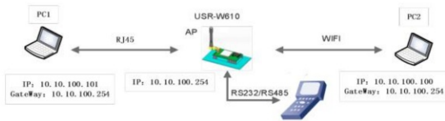
Figure 9 AP+LAN application
