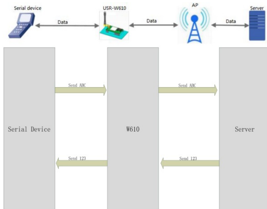
Figure 13 Transparent transmission mode
