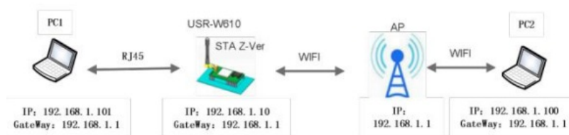
Figure 12 Bridge mode
