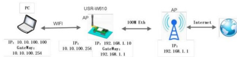
Figure 10 AP+WAN application
