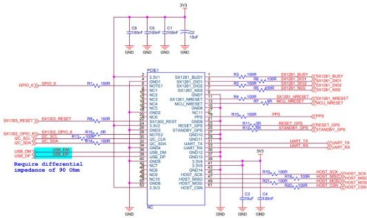
Figure 5: Schematic Diagram
