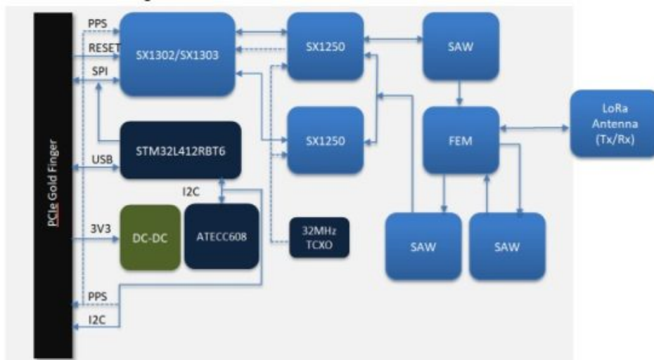
Figure 2: Block Diagram
