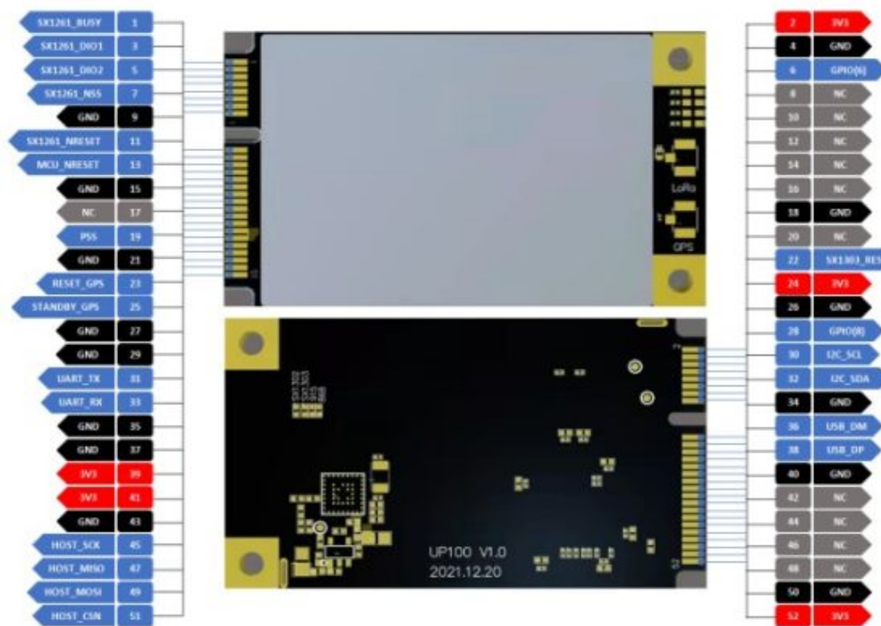
Figure 3: Pinout Diagram
