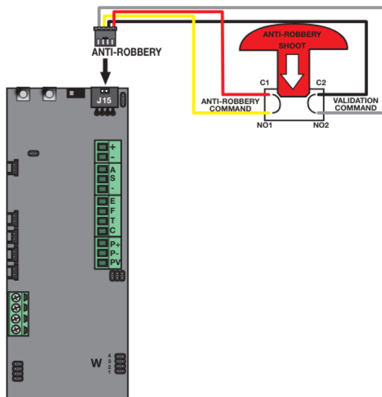
G – Example of connection of FAST 01 2C PRO PLUS outputs with antirobbery connection
