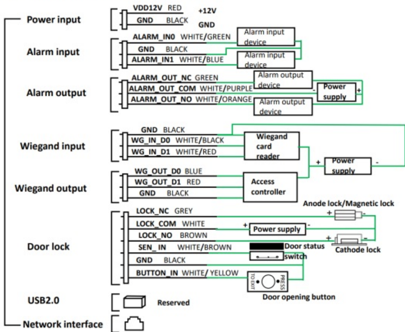
Figure 3-1 Wiring Schematic Diagrams
