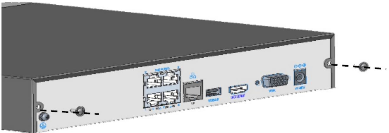
Figure 4-1 Rear Panel
