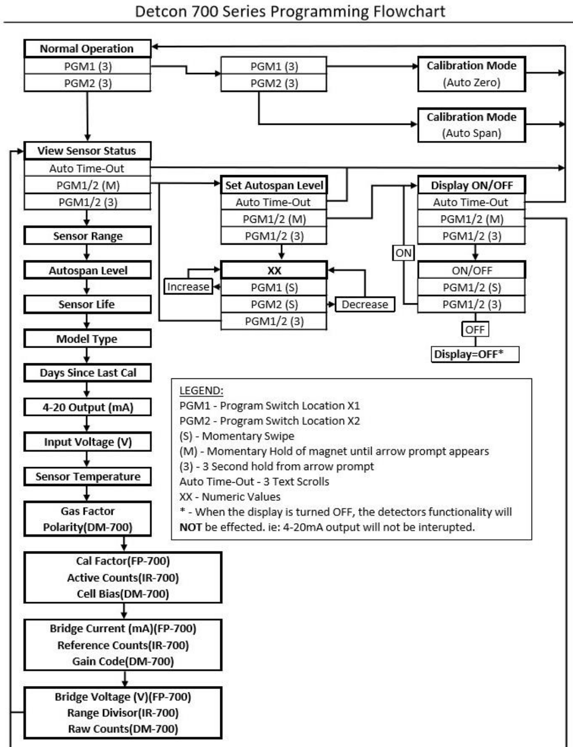
Figure 4: Detcon 700 Series Programming Flowchart
