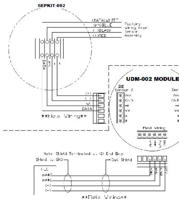
Figure 2: UDM Wiring Diagram
