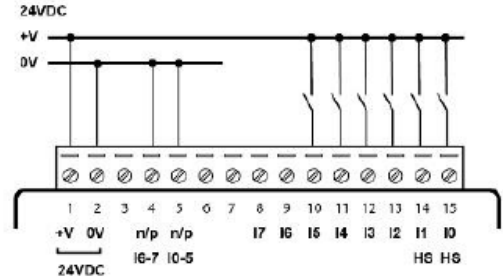
Input wiring (I0-I5), pnp (source)
