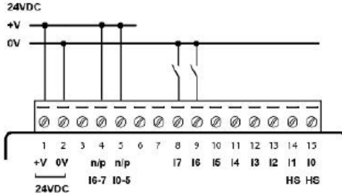
Input wiring (I6-I7), npn (sink)
