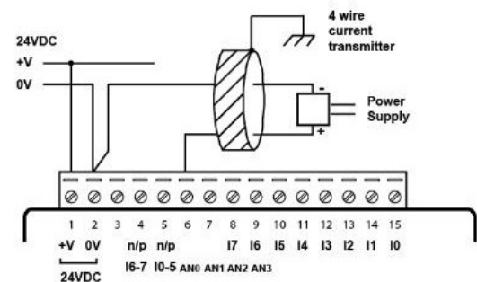
4-wire (AN0-AN1)
