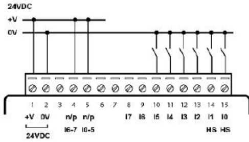
Input wiring (I0-I5), npn (sink)
