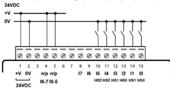
Input wiring (I0-I5), npn (sink)
