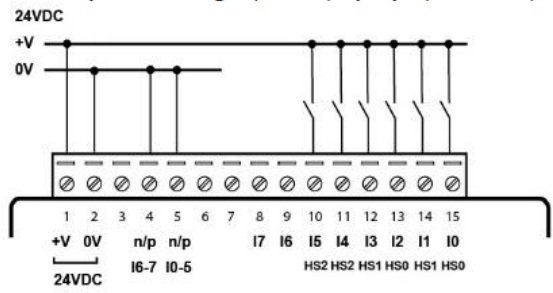
Input wiring (I0-I5), pnp (source)
