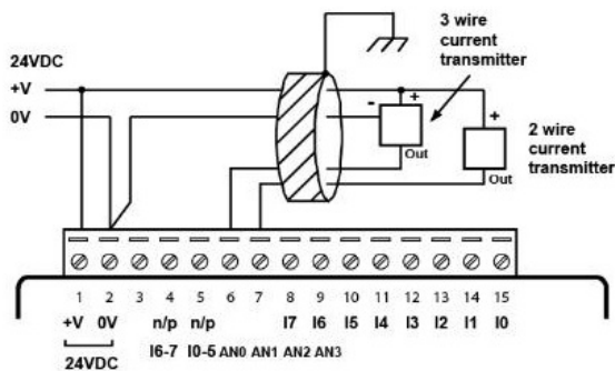
2 or 3-wire (AN0-AN1)
