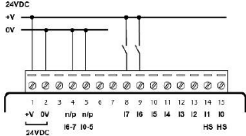
Input wiring (I6-I7), pnp (source)
