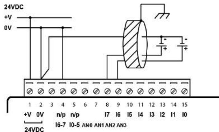
JZ20-R16/JZ20-J-R16/JZ20-J-R16HS (AN2-AN3)
