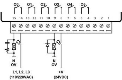
JZ20-R16/JZ20-J-R16/JZ20-J-R16HS
