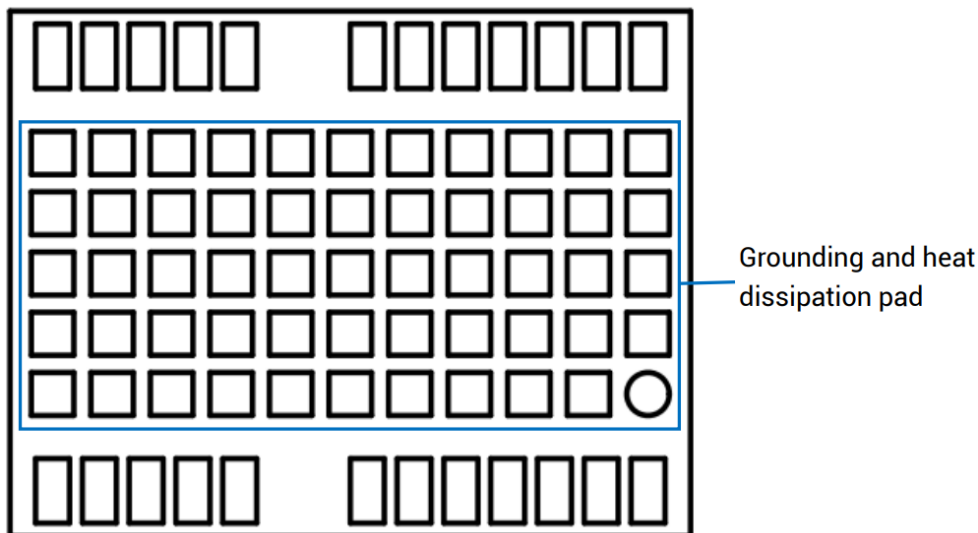
Figure 3-3 Grounding and Heat Dissipation Pad
