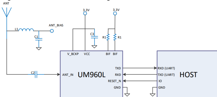
Figure 3-1 UM960L Minimal Design
