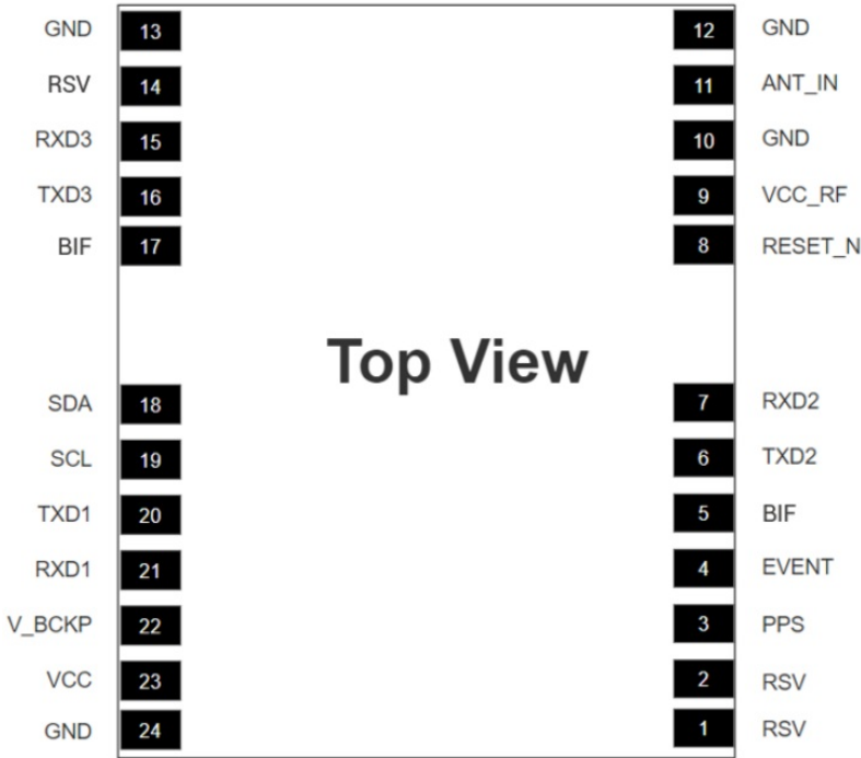
Figure 2-1 UM960L Pin Definition
