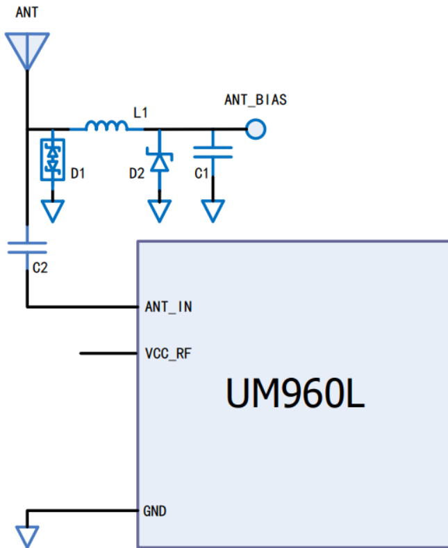
Figure 3-2 UM960L External Antenna Feed Reference Circuit
