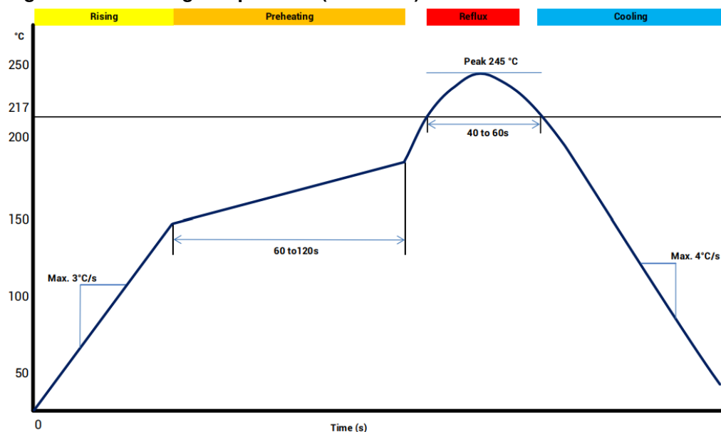
Figure 4-1 Soldering Temperature (Lead-free)
