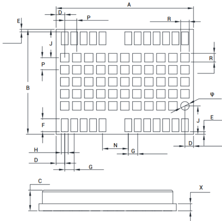
Figure 2-2 UM960L Mechanical Dimensions
