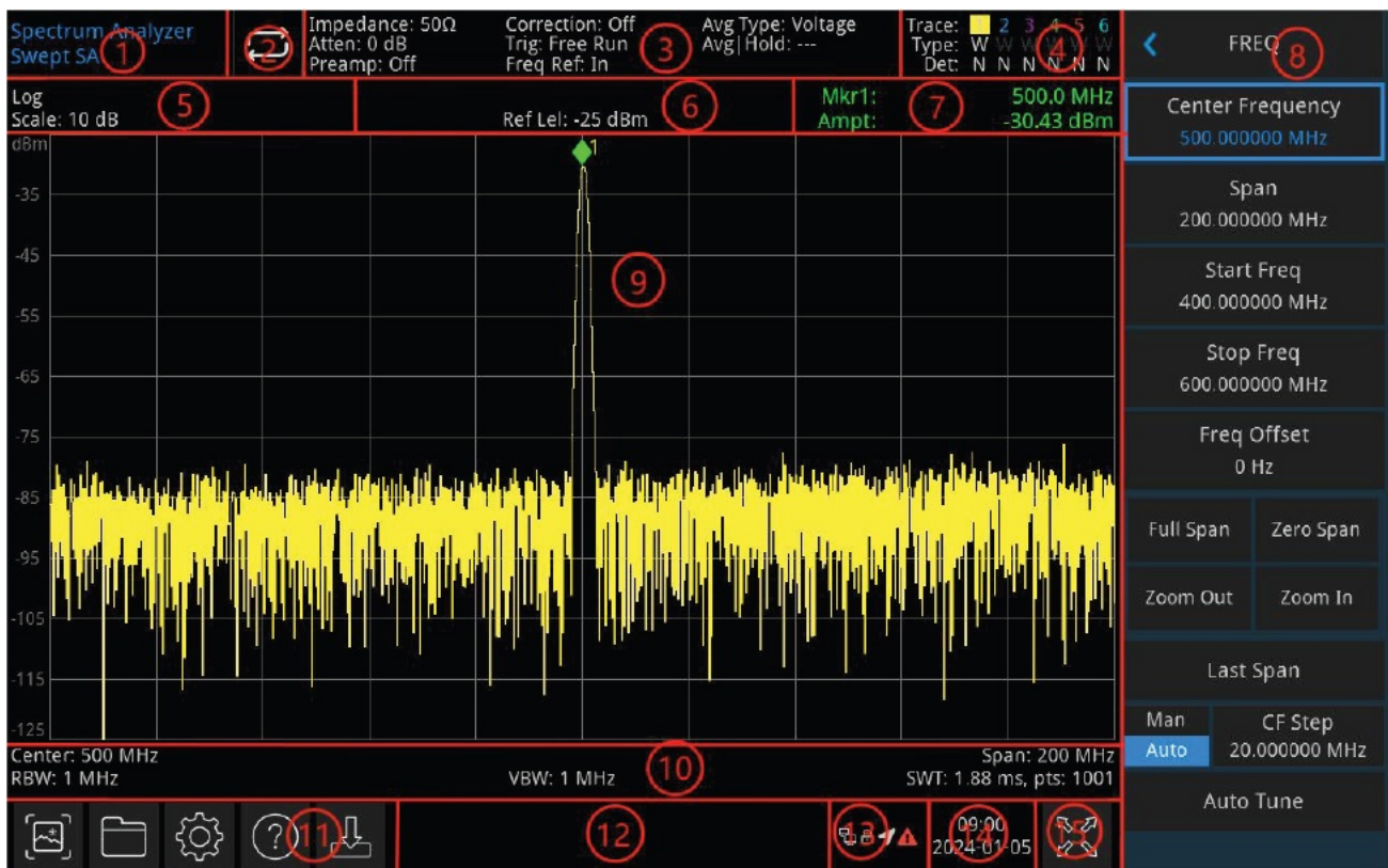
Figure 1-2 User Interface
