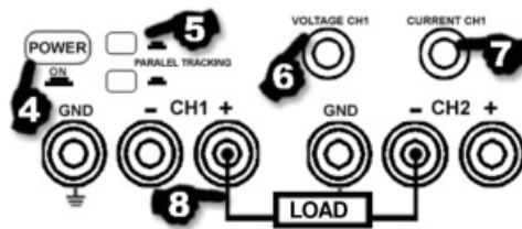
Figure 9 – Parallel Connection of the adjustable power supplies of the UTP3303 and UTP3305.
