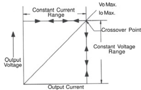
Figure 7 – Constant Voltage and Constant Current features.
