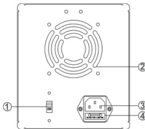
Figure 4 – Rear Panel: Models UTP1303 / UTP1305
