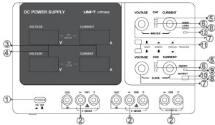
Figure 1 – Front Panel: Models UTP3303 / UTP3305
