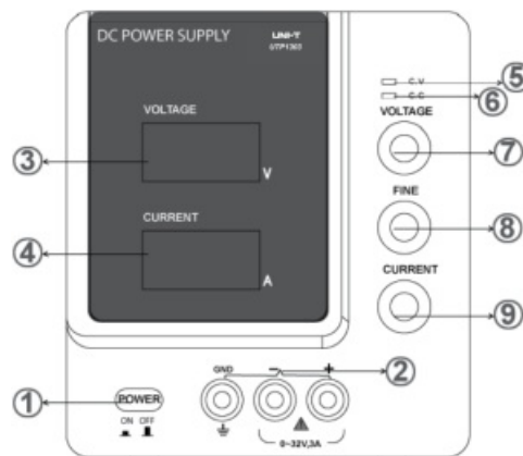
Figure 2 – Front Panel: Models UTP1303 / UTP1305
