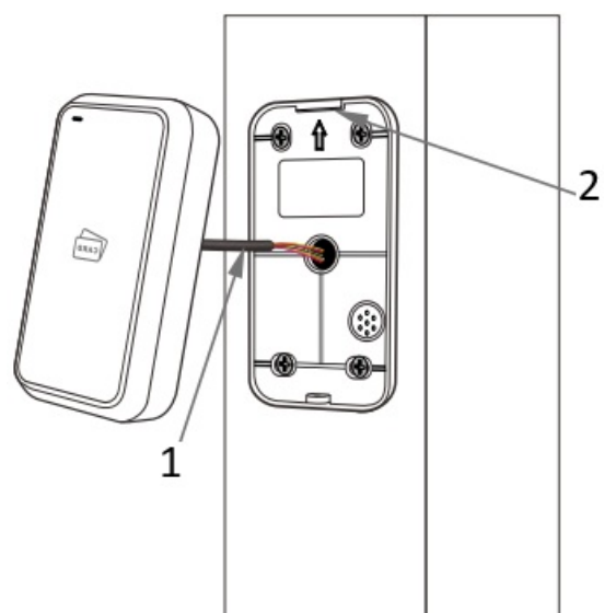
Figure 3 – Installation of Mounting Hardware
