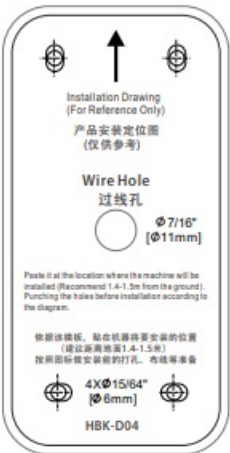
Installation Drawing x1
