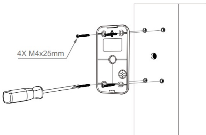
Figure 3 – Installation of Mounting Hardware
