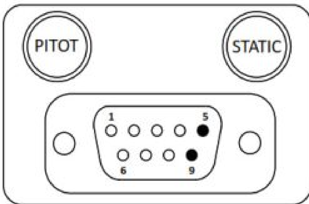
Figure 3 – Unit Connections – DB-9, Male Connector – Rear View
