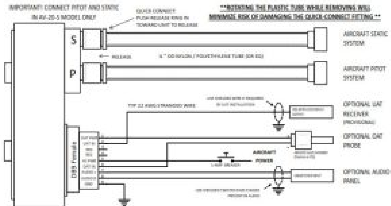
Figure 2 – Wiring Diagram
