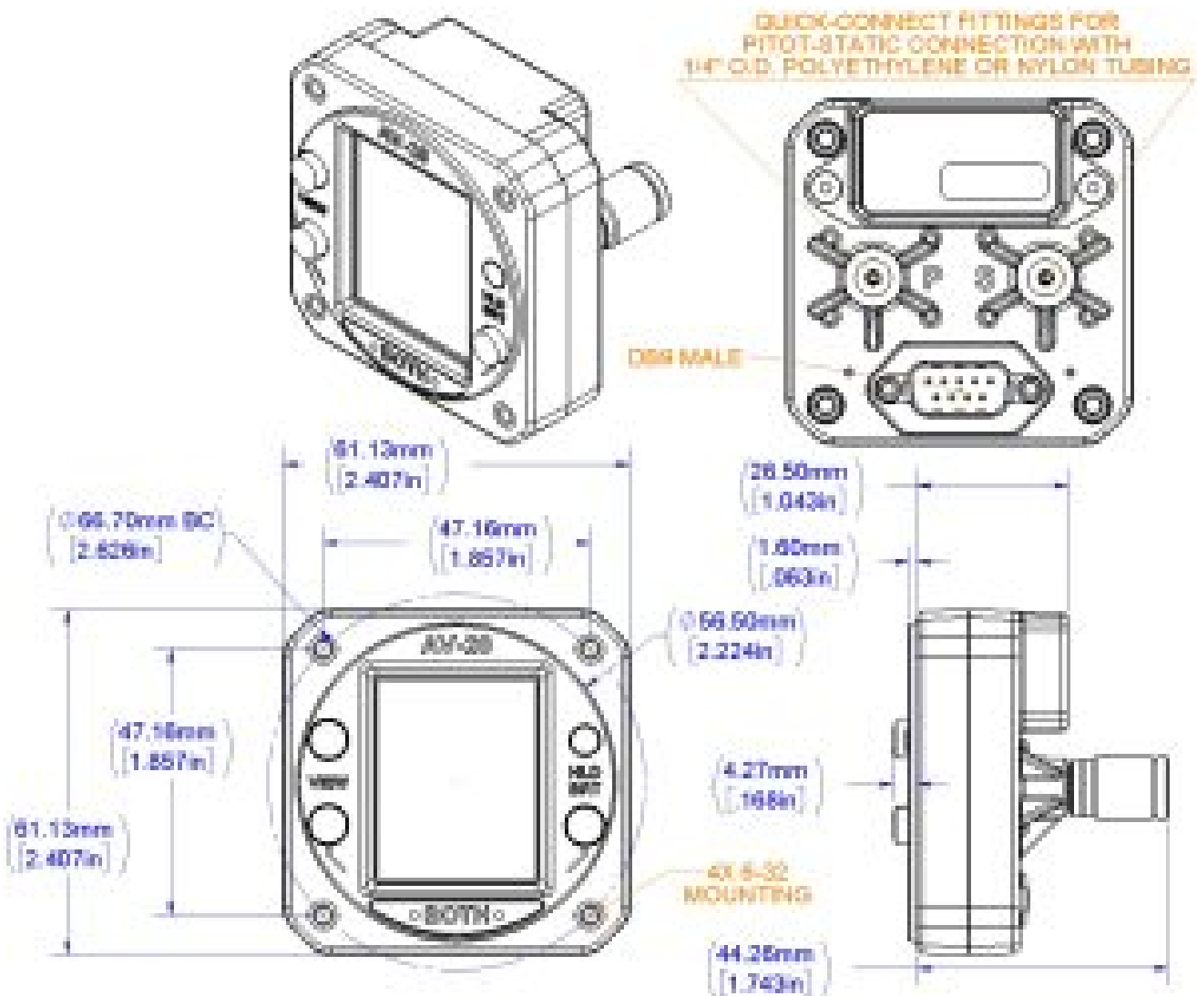
Figure 1 – Mechanical Drawing
