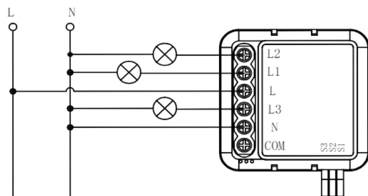
Single Control
