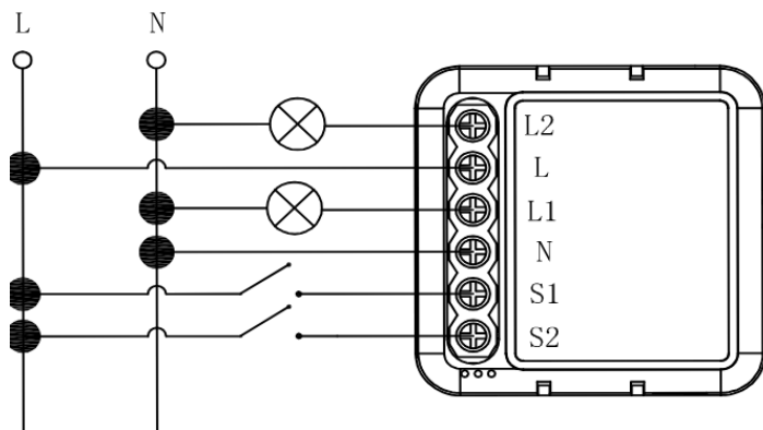
Double Switch[
