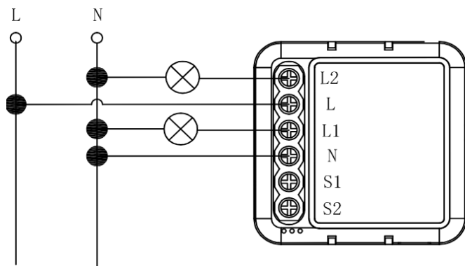
Single Control
