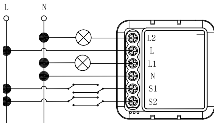
Double Switch[
