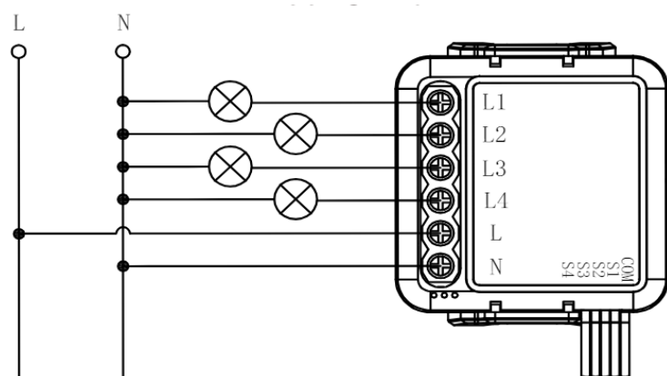
Single Control
