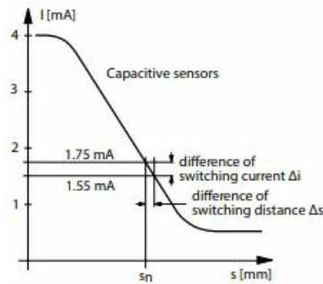
Abb. 1: NAMUR characteristic curve of the capacitive sensors as per EN 60947-5-6
