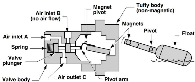
Figure 2: Low level operation – direct acting
