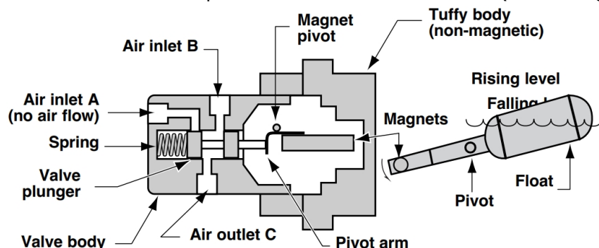
Figure 3: High level operation – direct acting
