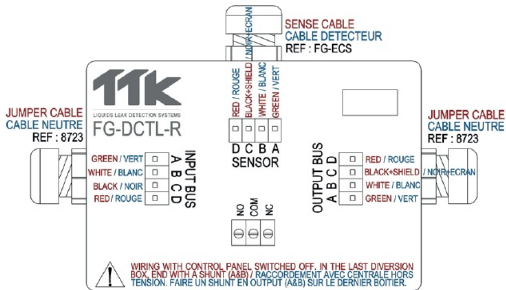
Figure 1.4.4.2: Interface box FG-DCTL-R cabling diagram
