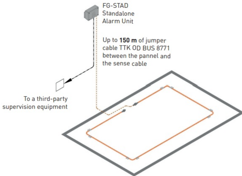
Figure 1.2.10 Layout with FG-STAD
