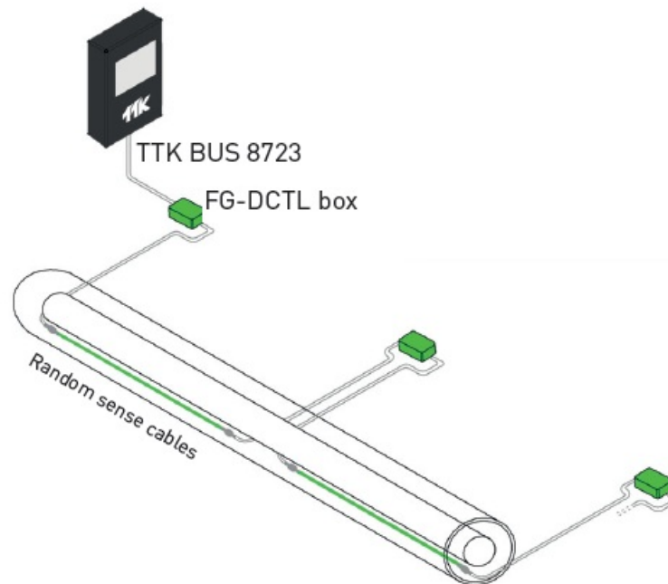
Figure 1.4.4 : Layout with FG-DCTL interface box
