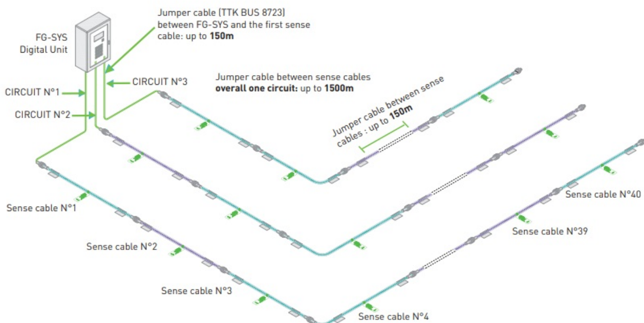
Figure 1.2.2 Basic layout of FG-SYS with 3 circuits
