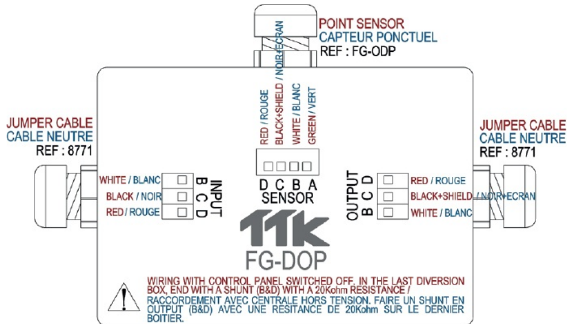
Figure 1.4.6 : Point sensor diversion box FG-DOP cabling diagram
