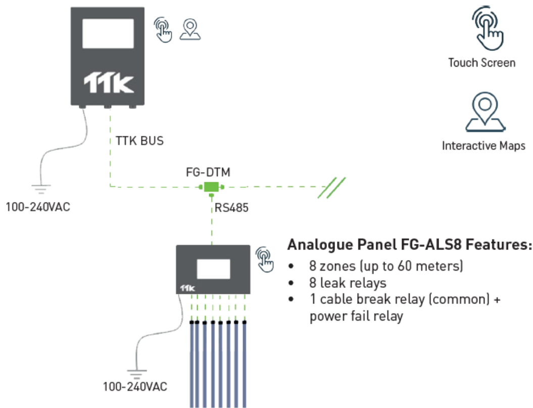
Figure 1.2.11.1 Basic layout of FG-DTM with FG-ALS8
