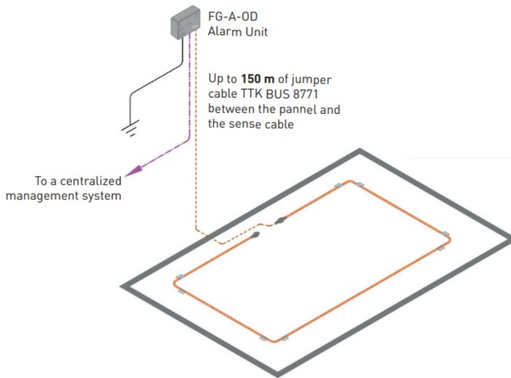
Figure 1.2.9 Layout with FG-A-OD
