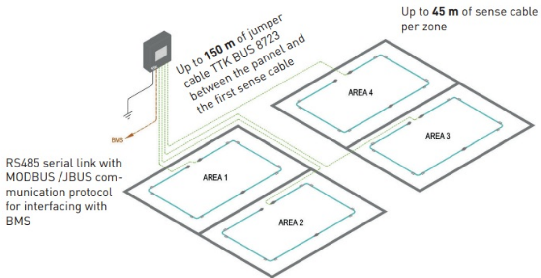
Figure 1.2.6 : Layout of FG-ALS4 with 4 zones
