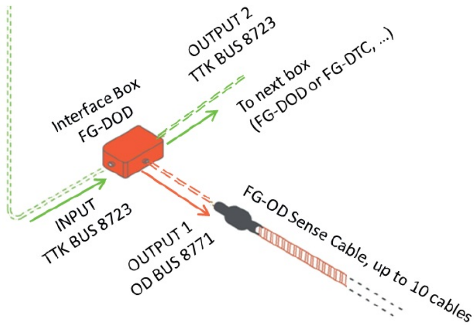
Figure 1.4.5.1: Connection of interface box FG-DOD
