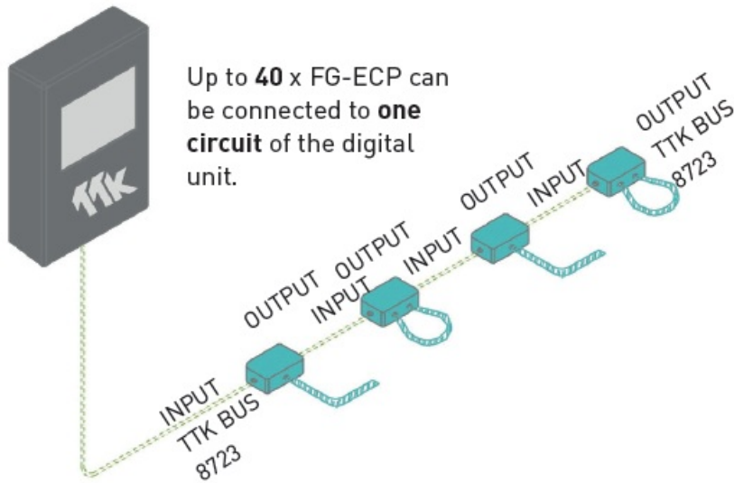
Figure 1.3.1: Layout of FG-ECP with FG-NET
