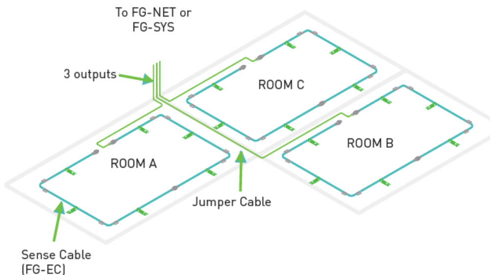
Figure 1.5 Horizontal layout
