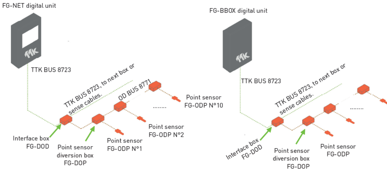
Figure 1.4.7 : Layout of mixed use of FG-DOD and FG-DOP boxes on FG-NET and FG-BBOX units
