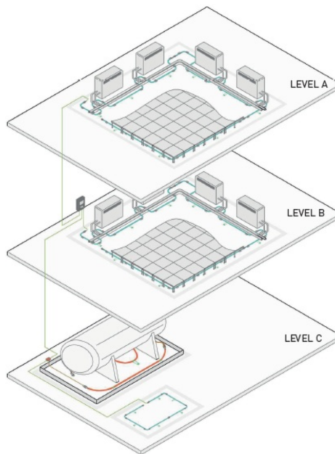
Figure 1.6 Vertical layout
