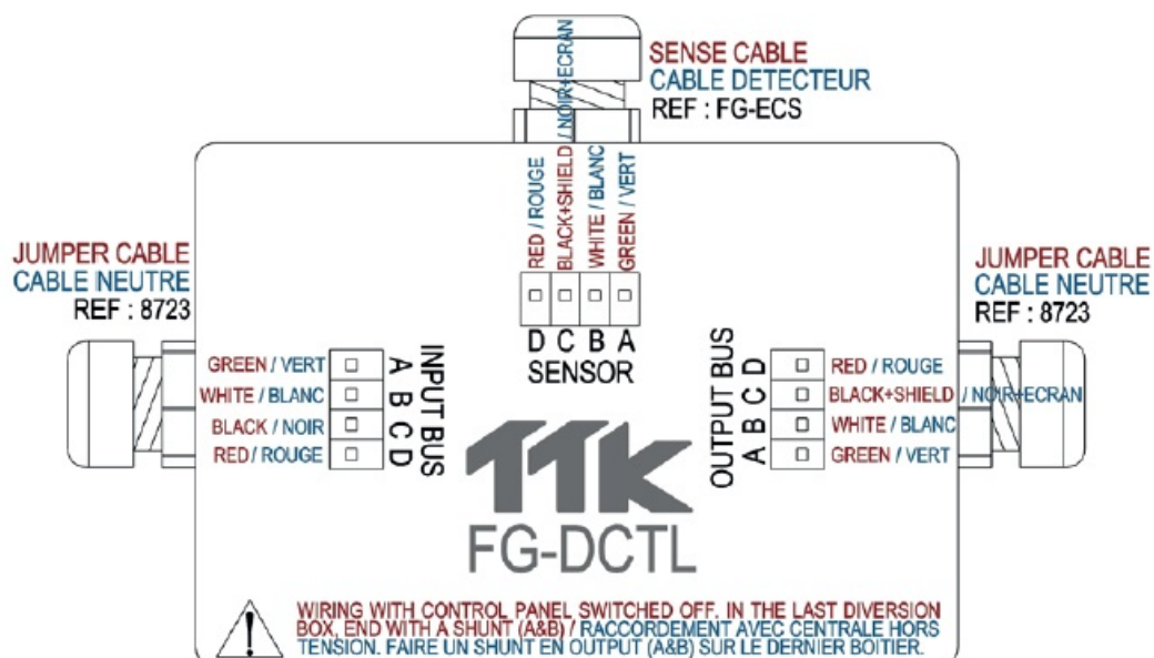
Figure 1.4.4.1: Interface box FG-DCTL cabling diagram
