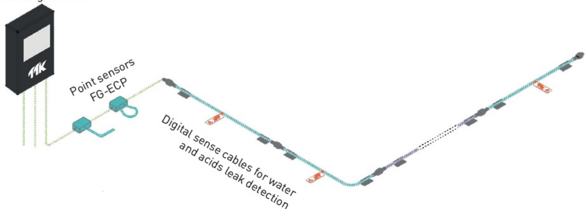
Figure 1.3.1.2: Layout of mixed connection of point sensors FG-ECP and digital sense cables FG-EC on a circuit of FG-NET digital unit
