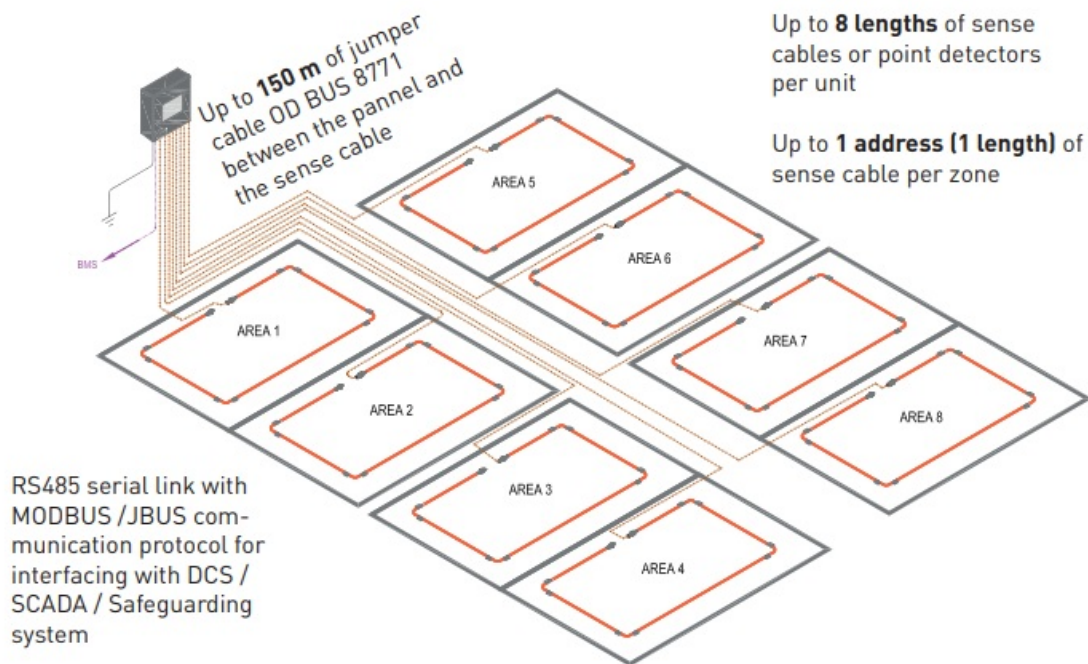
Figure 1.2.5 : Layout of FG-ALS8-OD with 8 zones
