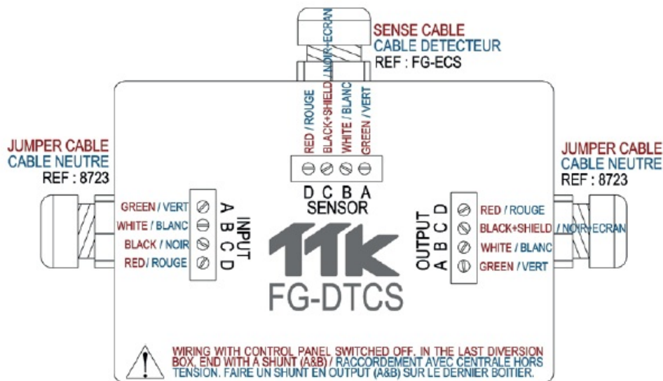
Figure 1.4.2.1: Addressable box FG-DTCS cabling diagram
