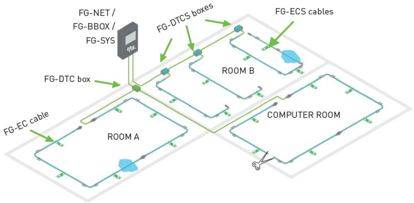
Figure 1.4.3 : Layout with FG-DTC et FG-DTCS boxes
