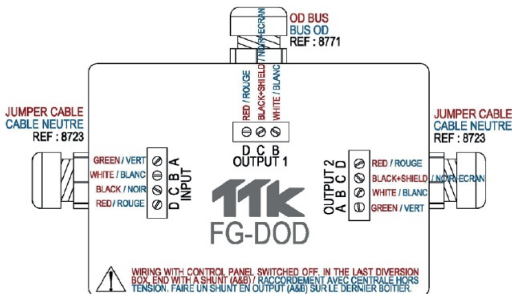
Figure 1.4.5 : Interface box FG-DOD cabling diagram
