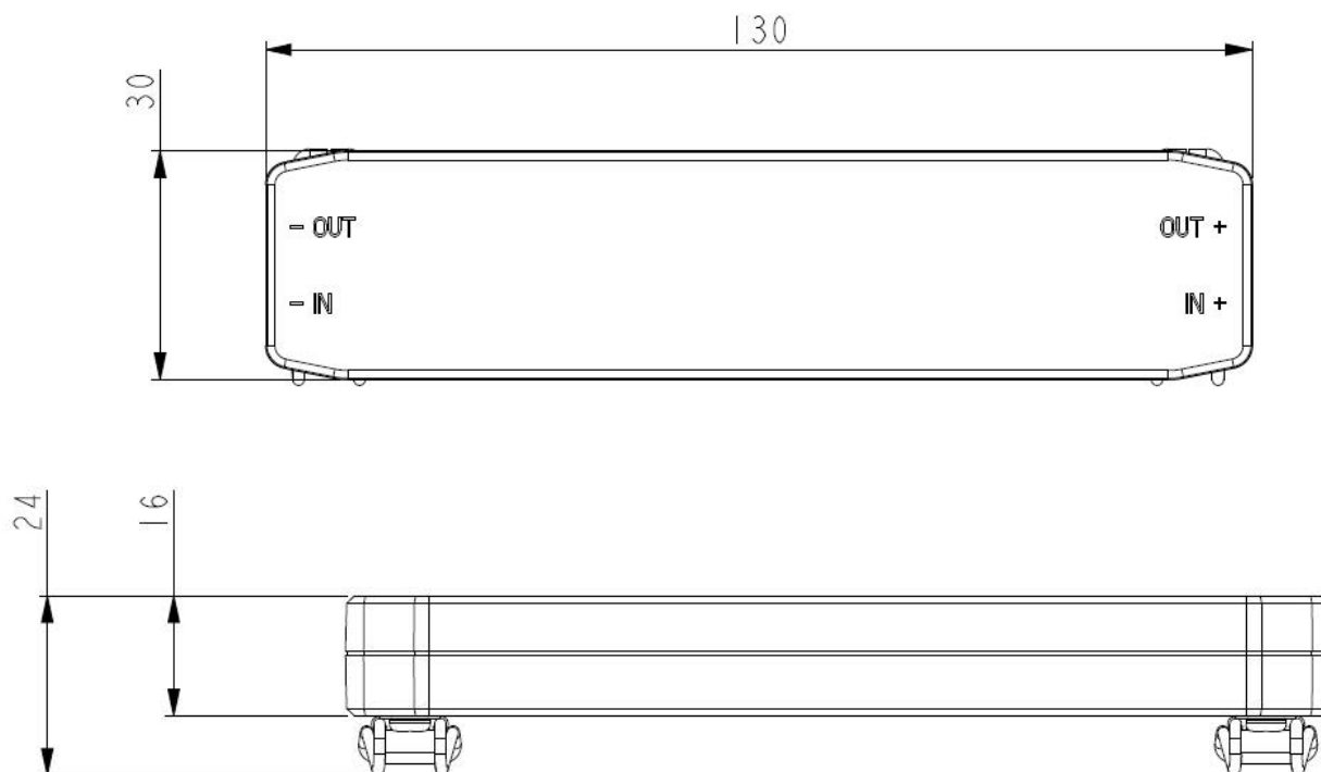
Figure 3.3&3.4&3.5 Dimensions of TSOL-RSDM-DS
