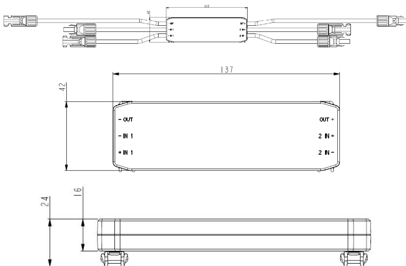
Figure 3.6&3.7&3.8 Dimensions of TSOL-RSDM-DD
