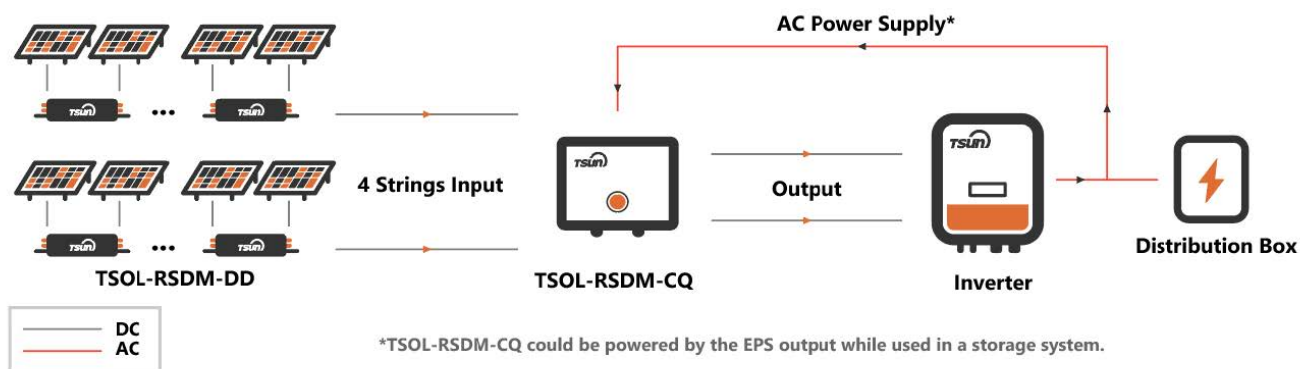
Figure 3.2 System Diagram (TSOL-RSDM-DD and TSOL-RSDM-CQ)
