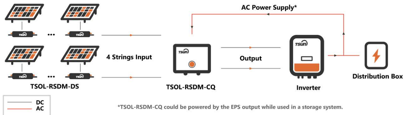
Figure 3.1 System Diagram (TSOL-RSDM-DS and TSOL-RSDM-CQ)
