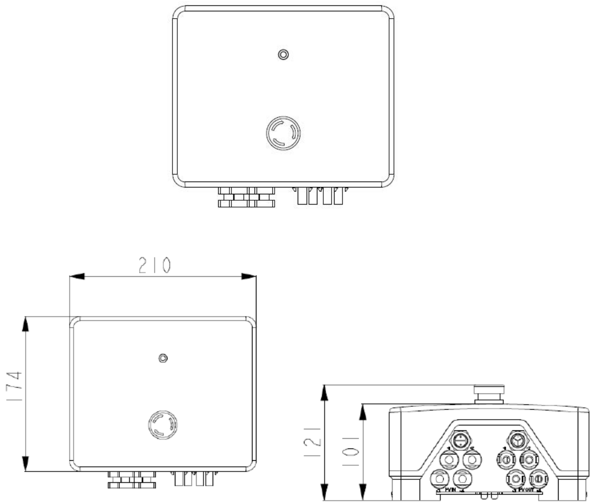
Figure 3.9&3.10&3.11.5 Dimensions of TSOL-RSDM-CQ
