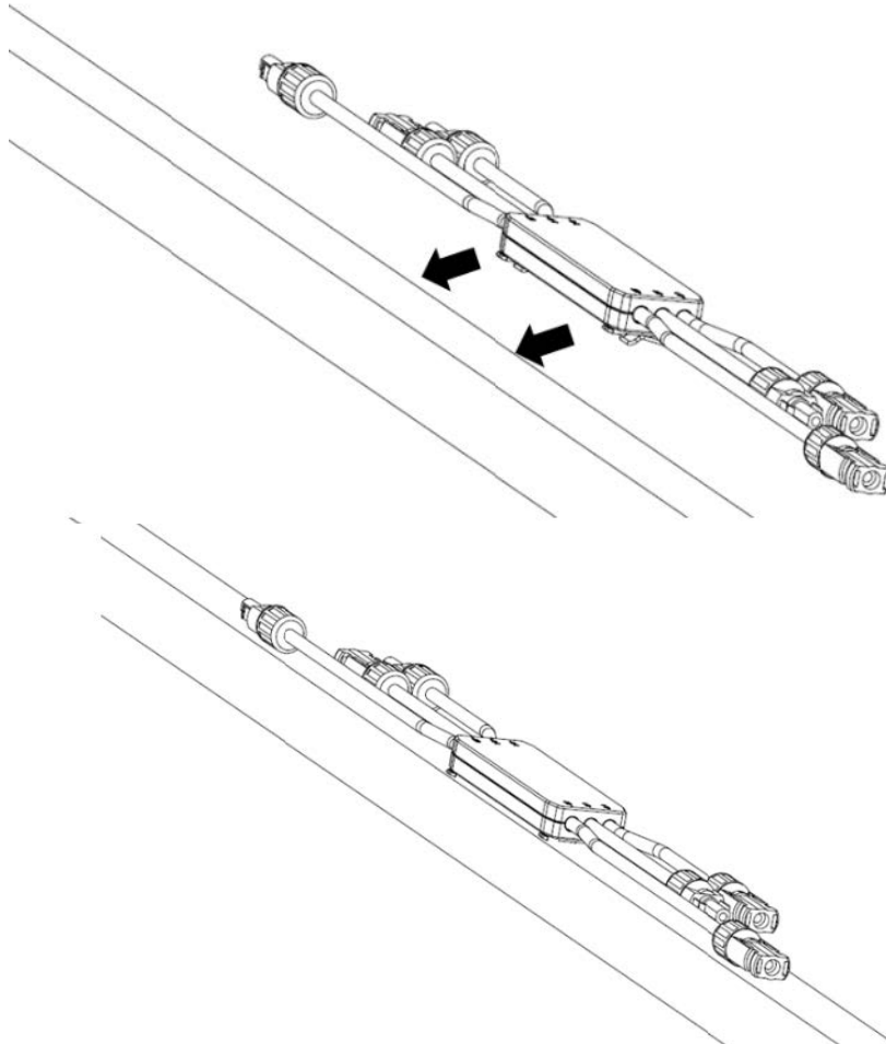
Figure 4.1&4.2 Fixing the Rapid Shutdown Device
