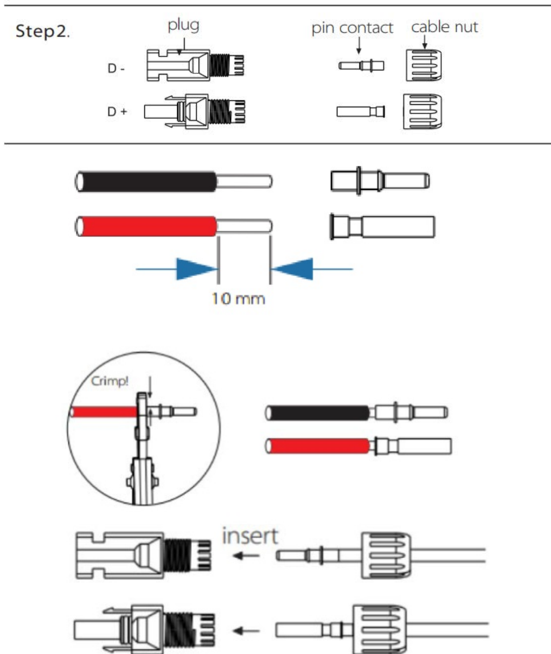
Figure 4.9&4.110&4.11&4.12 Make the DC cable
