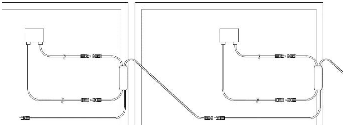
Figure 4.5 Connecting Rapid Shutdown Device in Series
