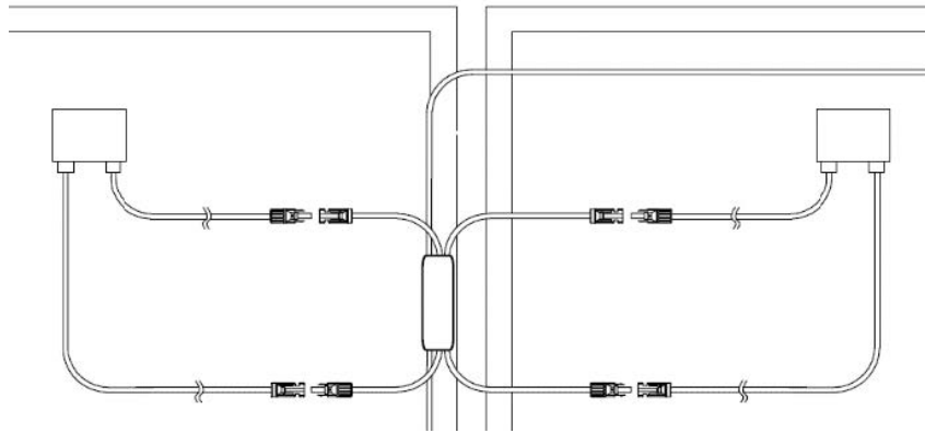
Figure 4.4 Connecting TSOL-RSDM-DD and solar modules
